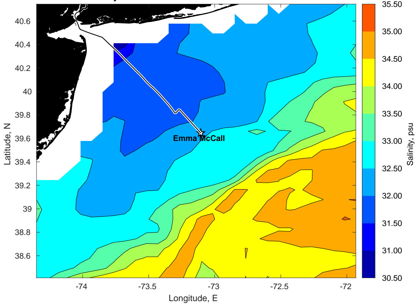
Surface Salinity for Emma McCall at 01-Jun-2023 00:00:00
