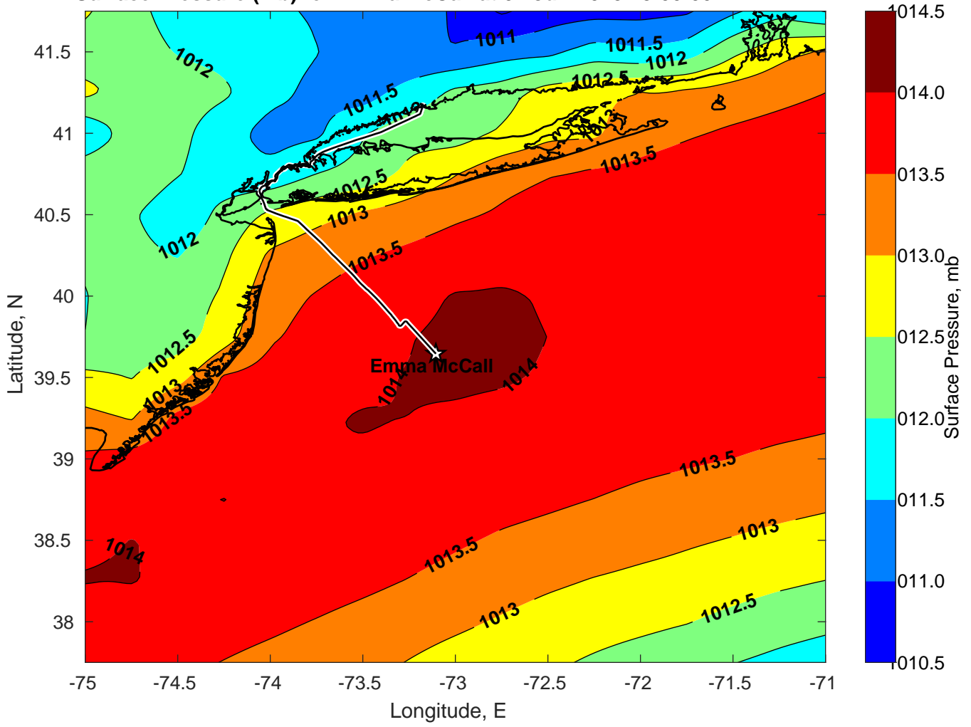
Surface Pressure (mb) for Emma McCall at 02-Jun-2023 18:00:00
