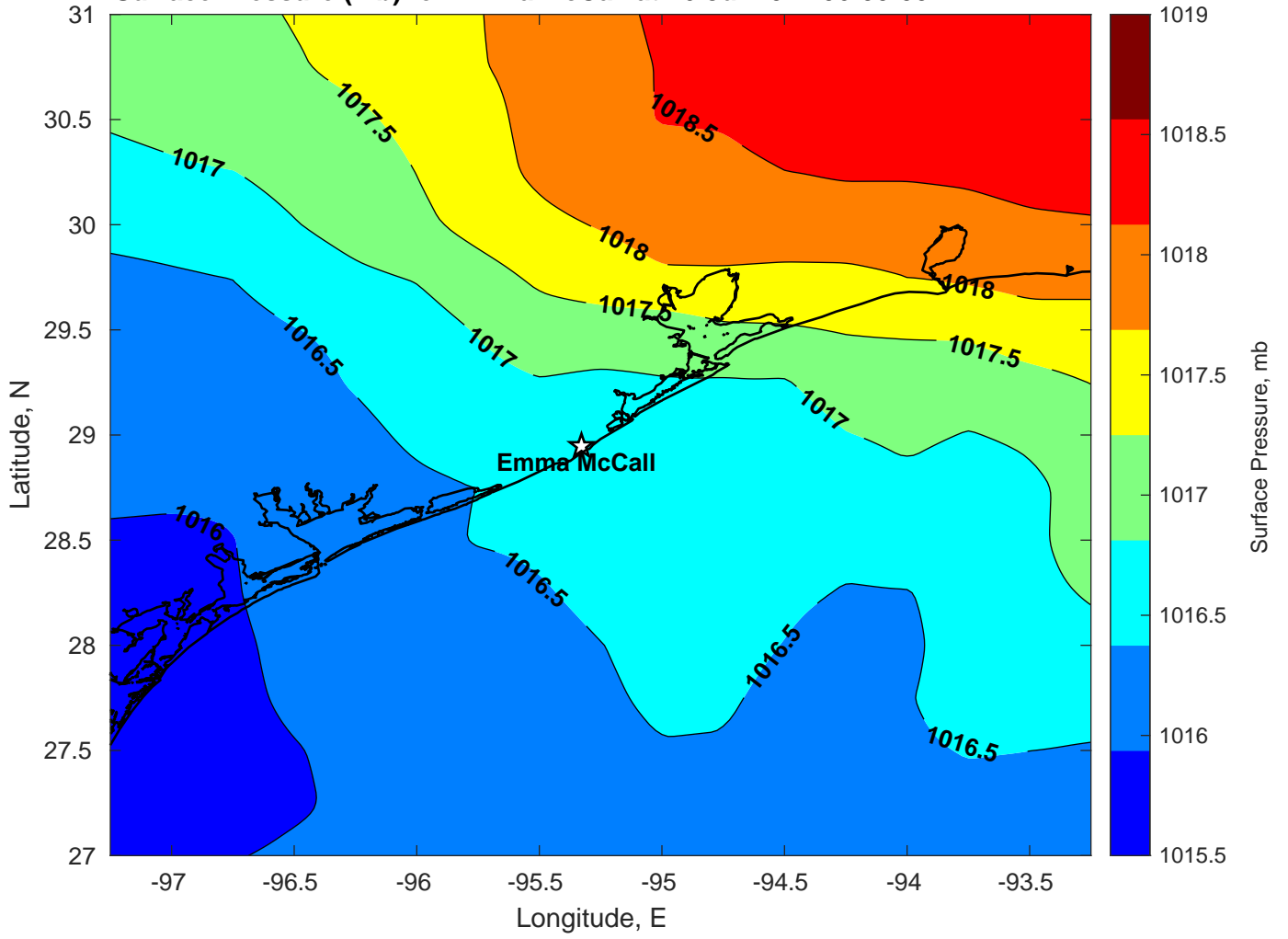
Surface Pressure (mb) for Emma McCall at 26-Jul-2024 06:00:00
