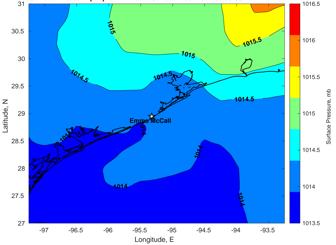
Surface Pressure (mb) for Emma McCall at 27-Jul-2024 06:00:00
