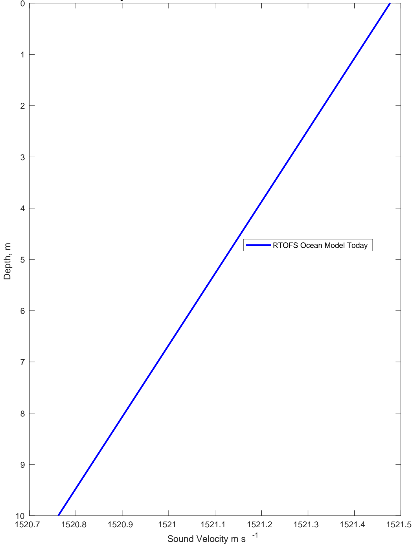
Sound Velocity Profile for Emma McCall on 16-Oct-2021 00:00:00
