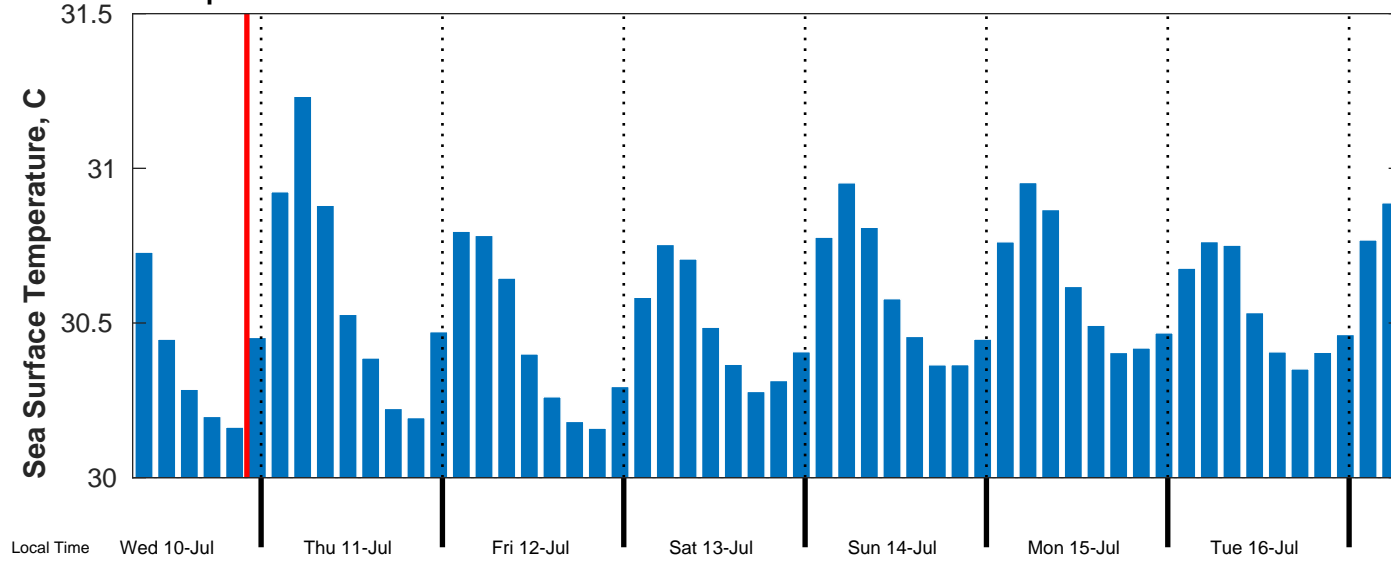
Sea Surface Temperature Forecast for Emma McCall from 11-Jul-2024 00:00:00 to 18-Jul-2024 00:00:00
