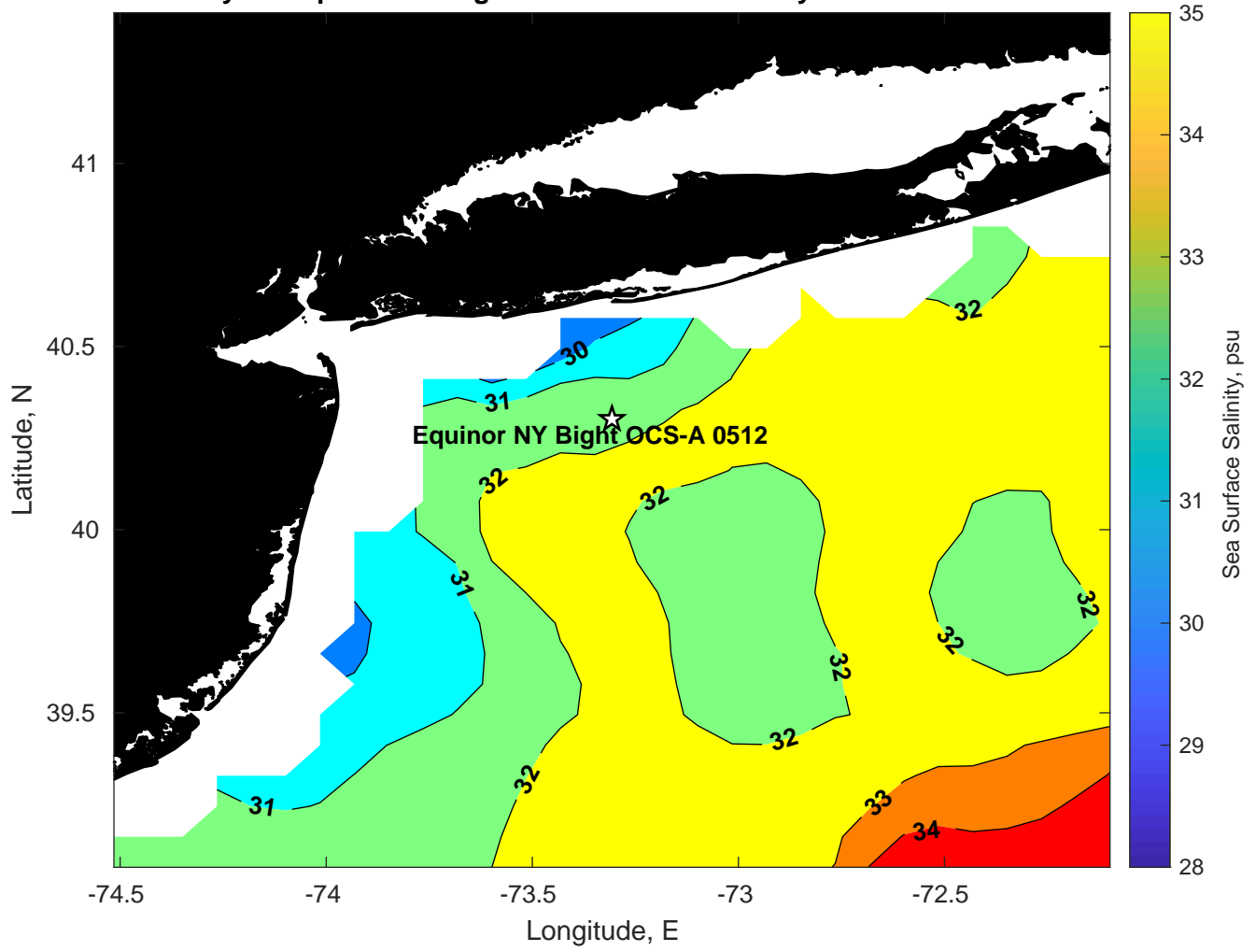
Surface Salinity for Equinor NY Bight OCS-A 0512 at 09-May-2024 00:00:00
