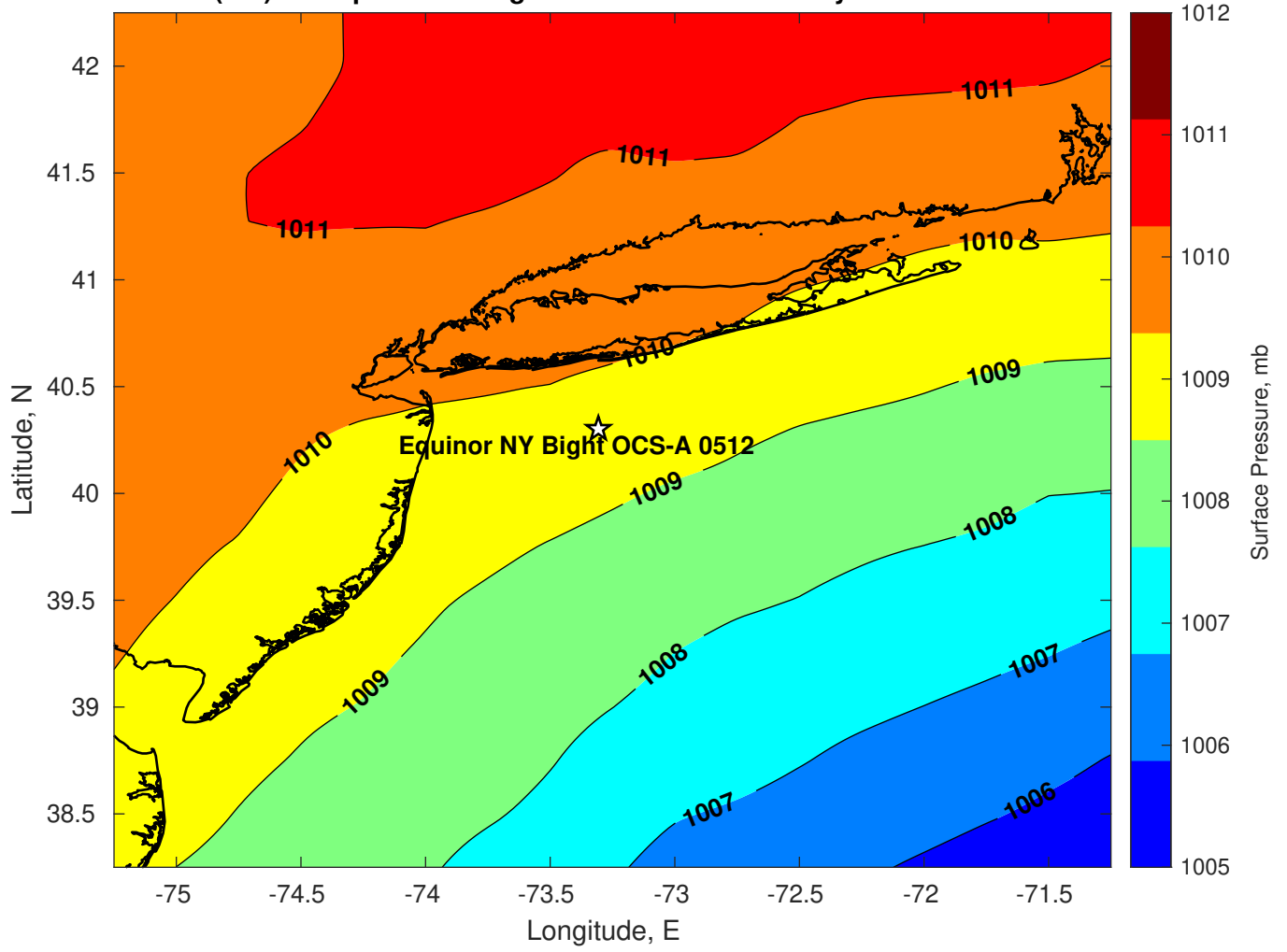
Surface Pressure (mb) for Equinor NY Bight OCS-A 0512 at 11-May-2024 12:00:00
