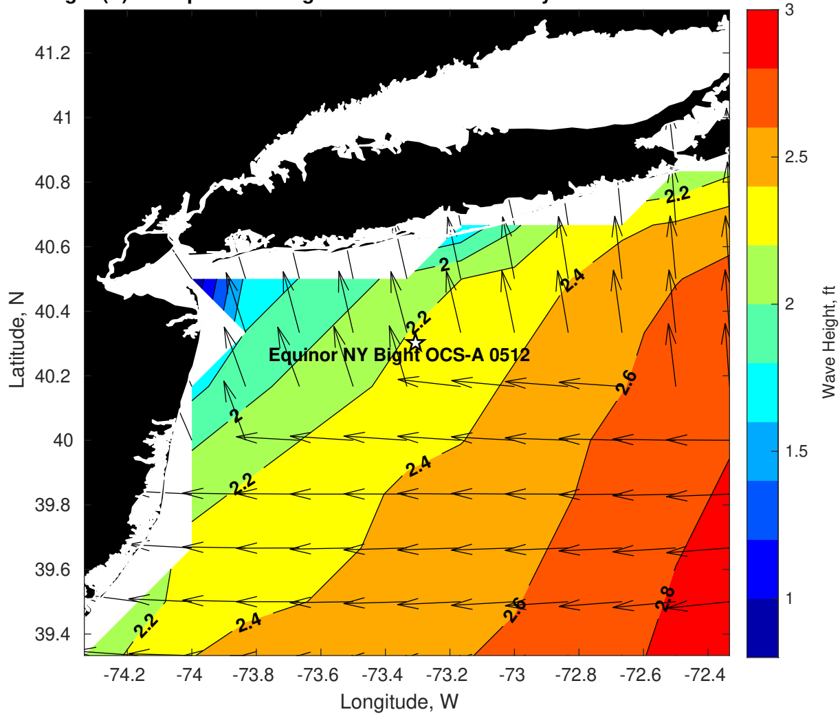
Wave Height (ft) for Equinor NY Bight OCS-A 0512 at 09-May-2024 18:00:00
