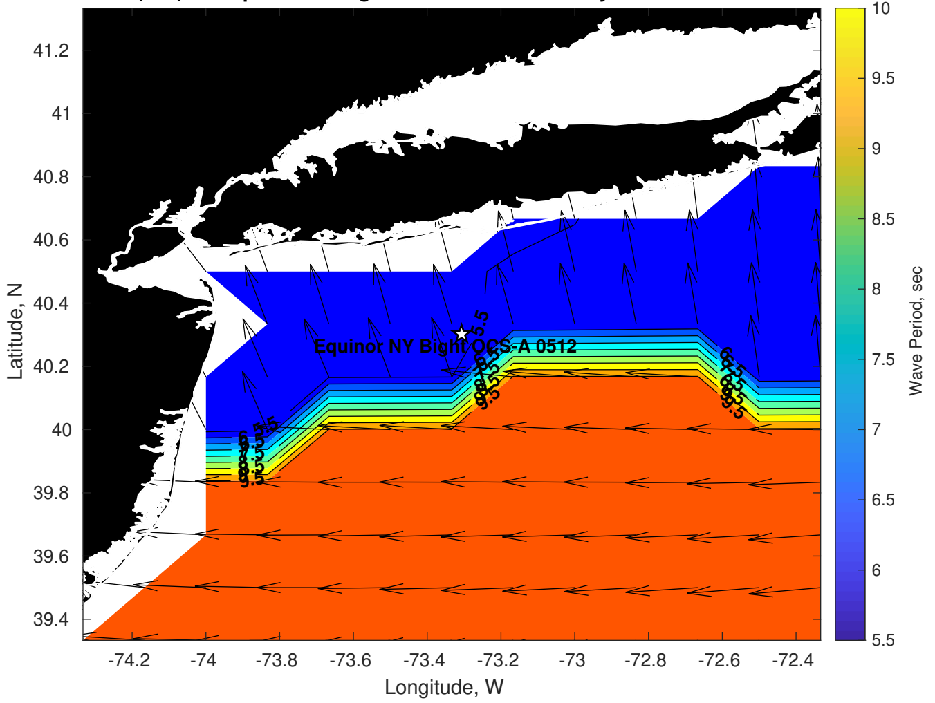
Wave Period (sec) for Equinor NY Bight OCS-A 0512 at 09-May-2024 18:00:00
