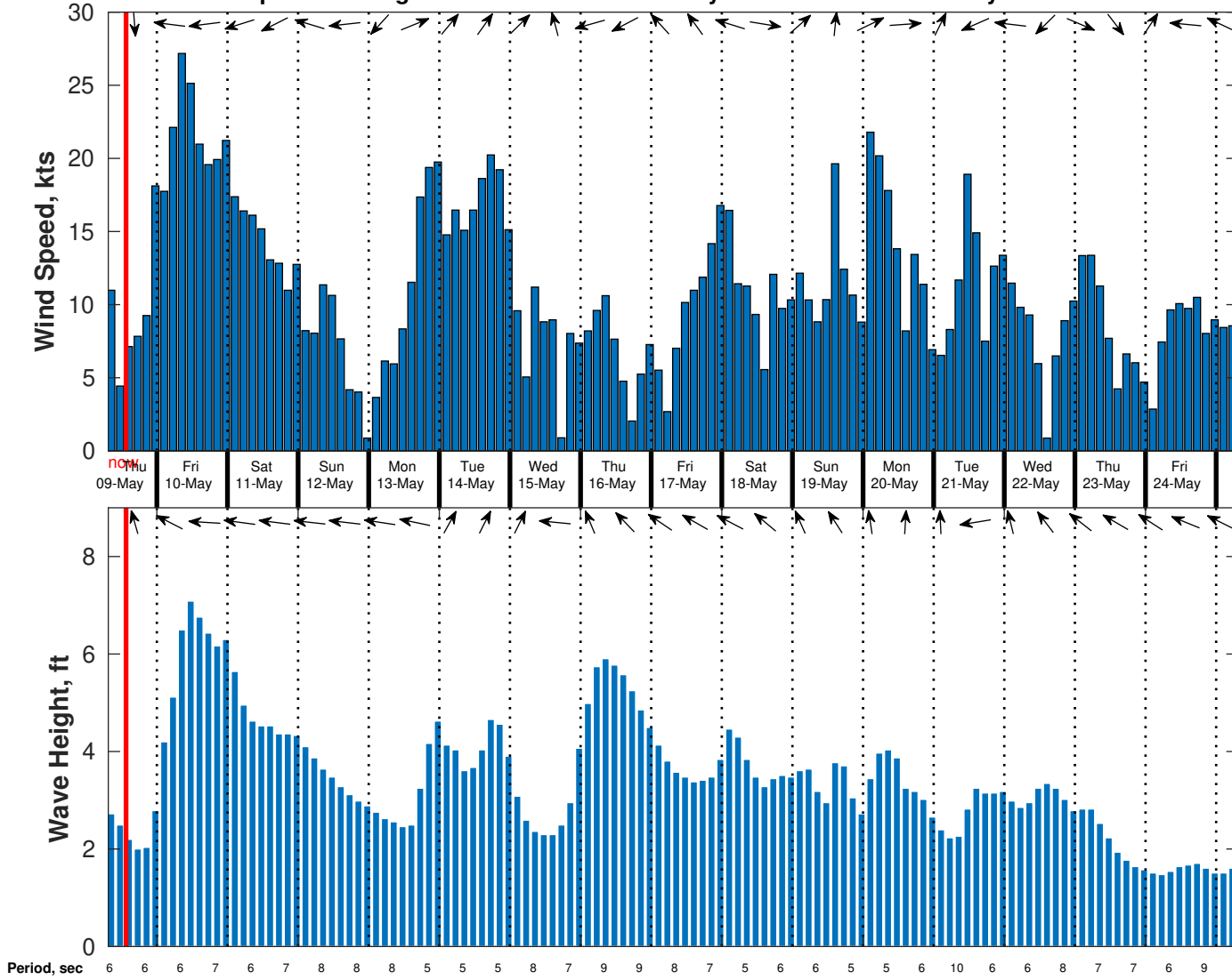
Wind & Wave Forecast for Equinor NY Bight OCS-A 0512 from 09-May-2024 07:00:00 to 25-May-2024 07:00:00
