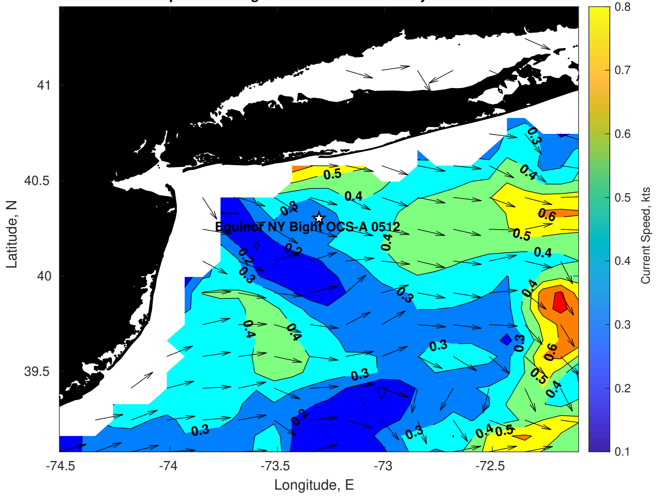
Surface Currents for Equinor NY Bight OCS-A 0512 at 09-May-2024 00:00:00
