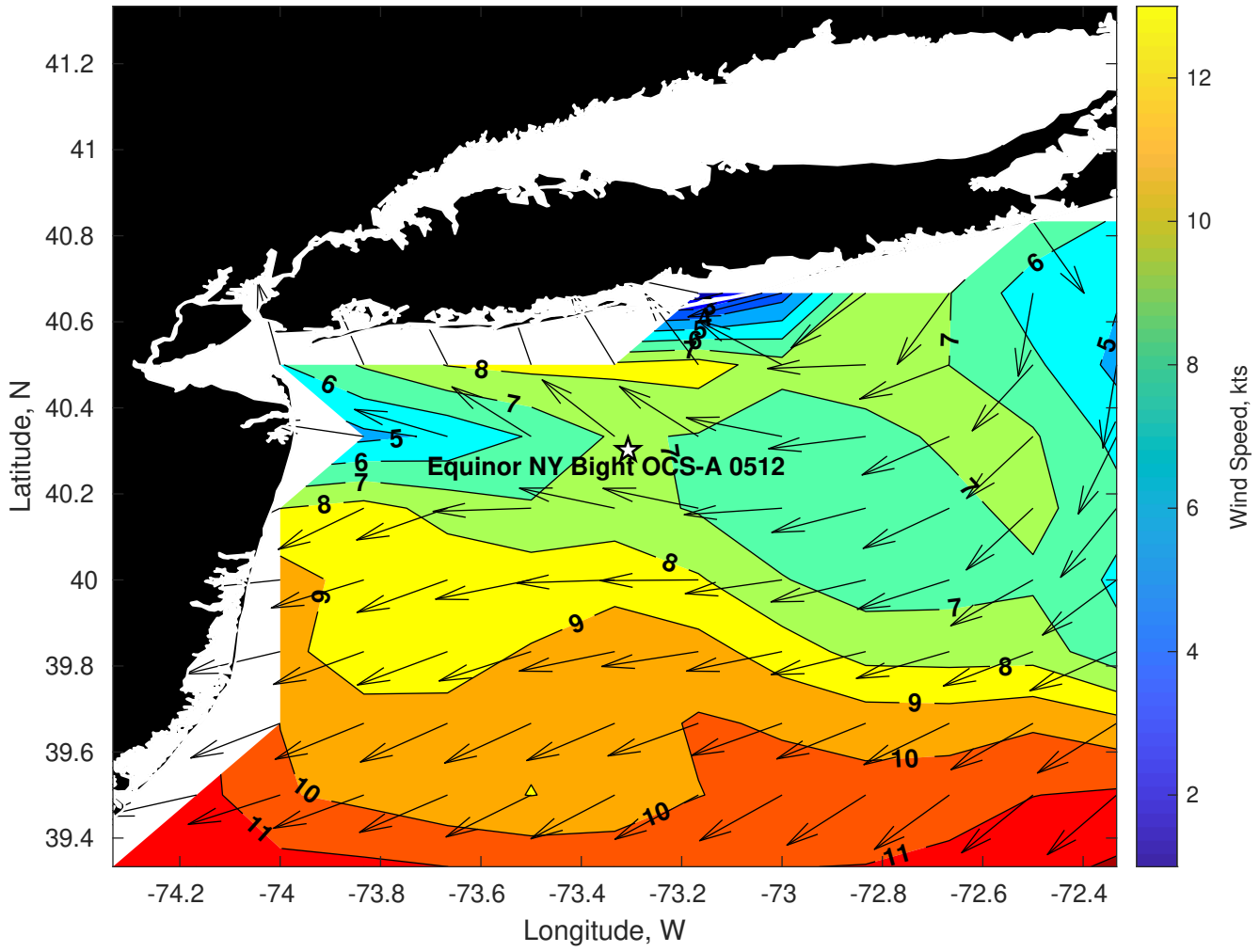
Winds (kts) for Equinor NY Bight OCS-A 0512 at 09-May-2024 18:00:00
