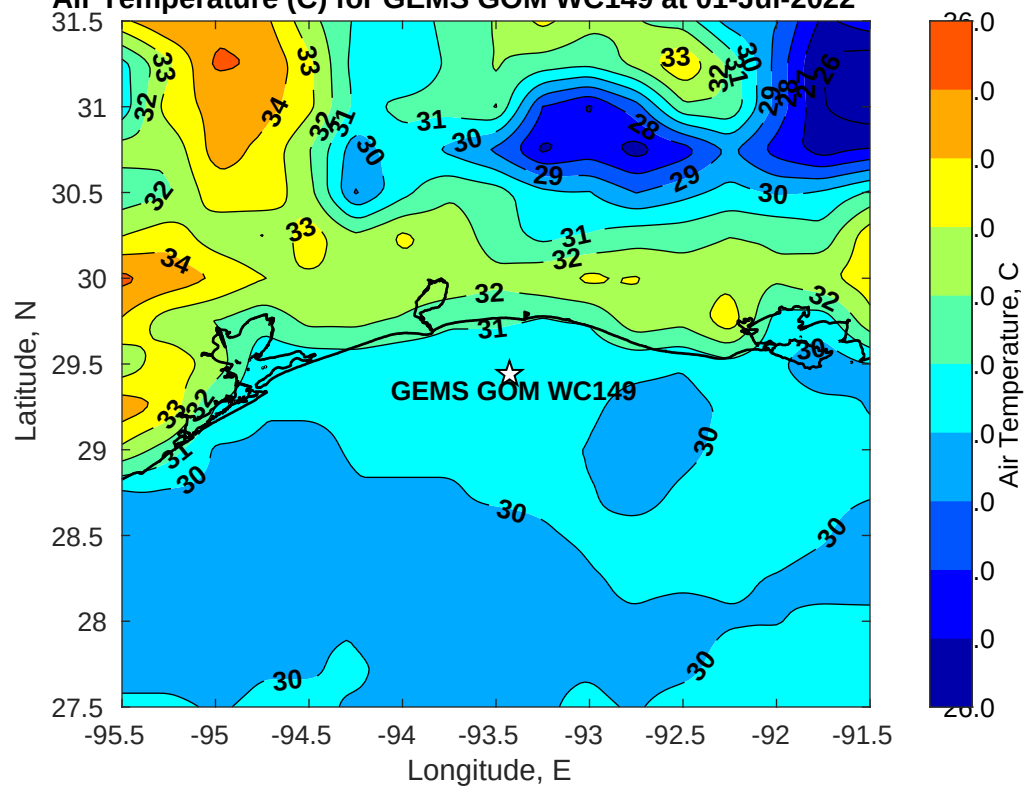
Air Temperature (C) for GEMS GOM WC149 at 01-Jul-2022
