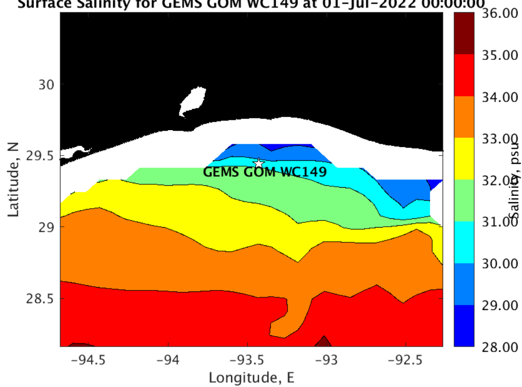
Surface Salinity for GEMS GOM WC149 at 01-Jul-2022 00:00:00
