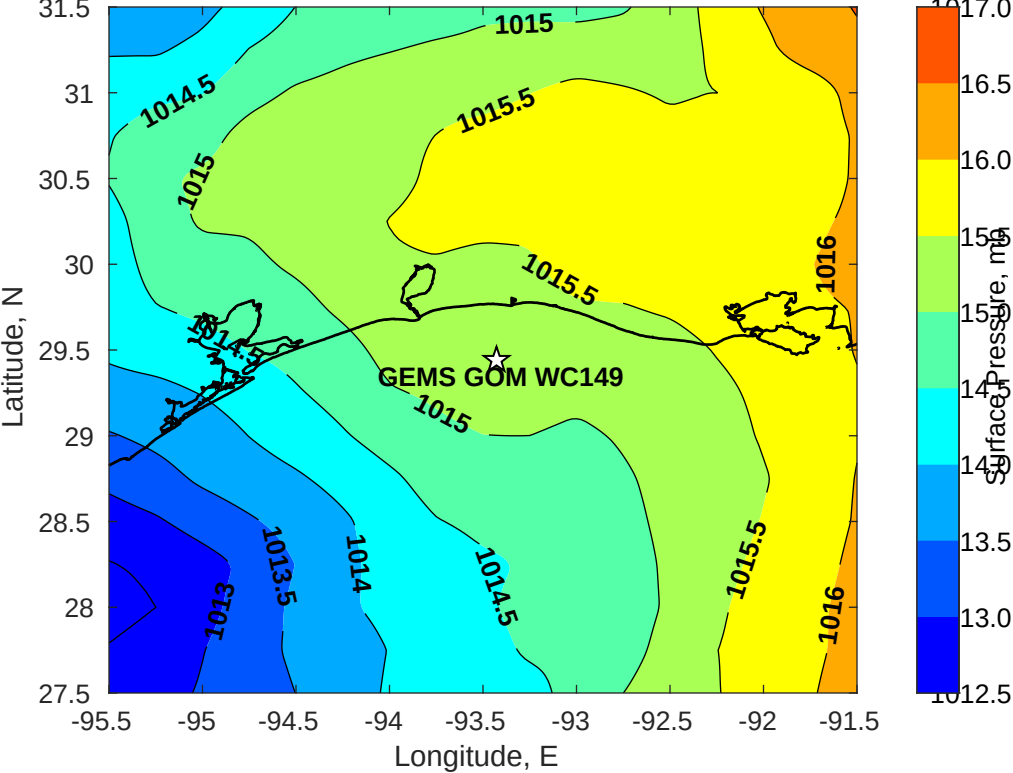
Surface Pressure (mb) for GEMS GOM WC149 at 01-Jul-2022 00:00:00
