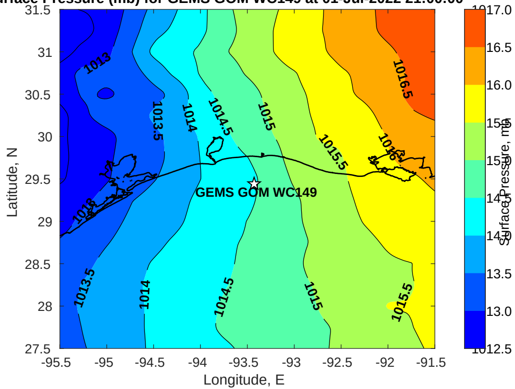
Surface Pressure (mb) for GEMS GOM WC149 at 01-Jul-2022 21:00:00
