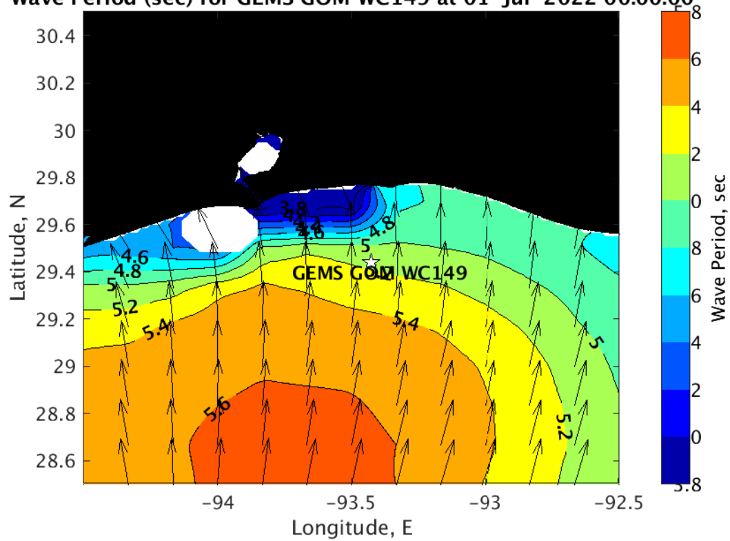
Wave Period (sec) for GEMS GOM WC149 at 01-Jul-2022 00:00:00
