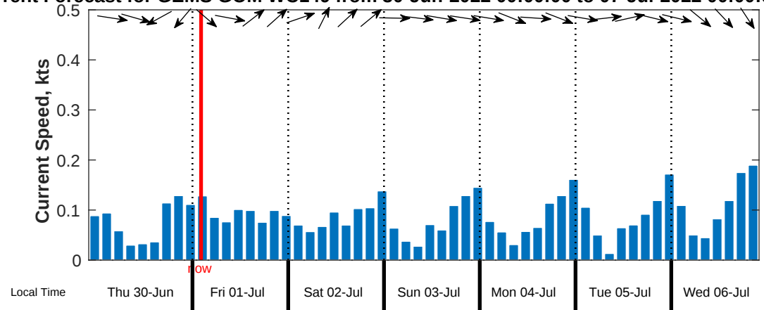
Current Forecast for GEMS GOM WC149 from 30-Jun-2022 00:00:00 to 07-Jul-2022 00:00:00
