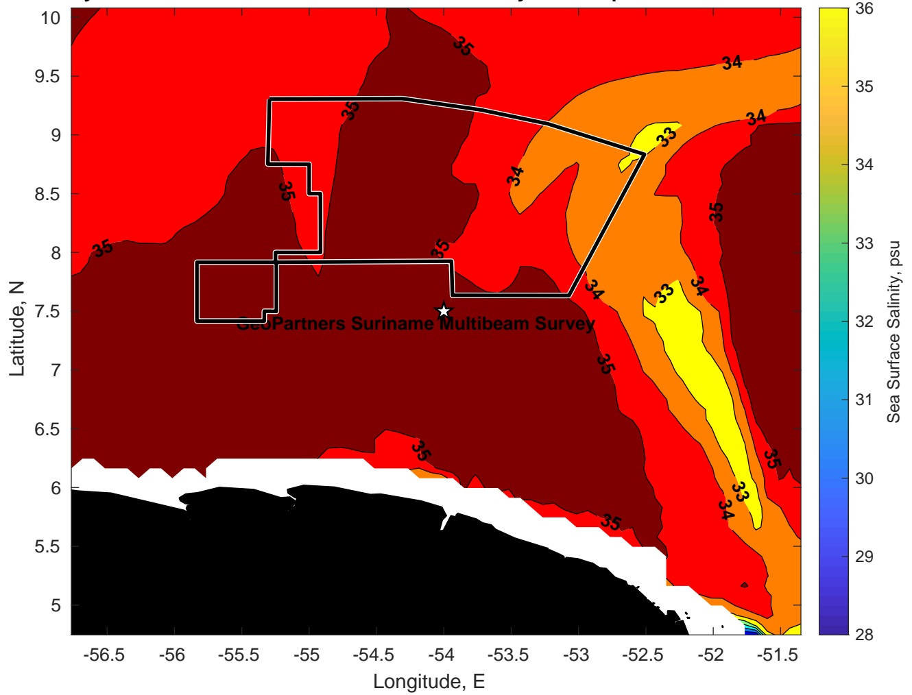
Surface Salinity for GeoPartners Suriname Multibeam Survey at 08-Sep-2024 00:00:00
