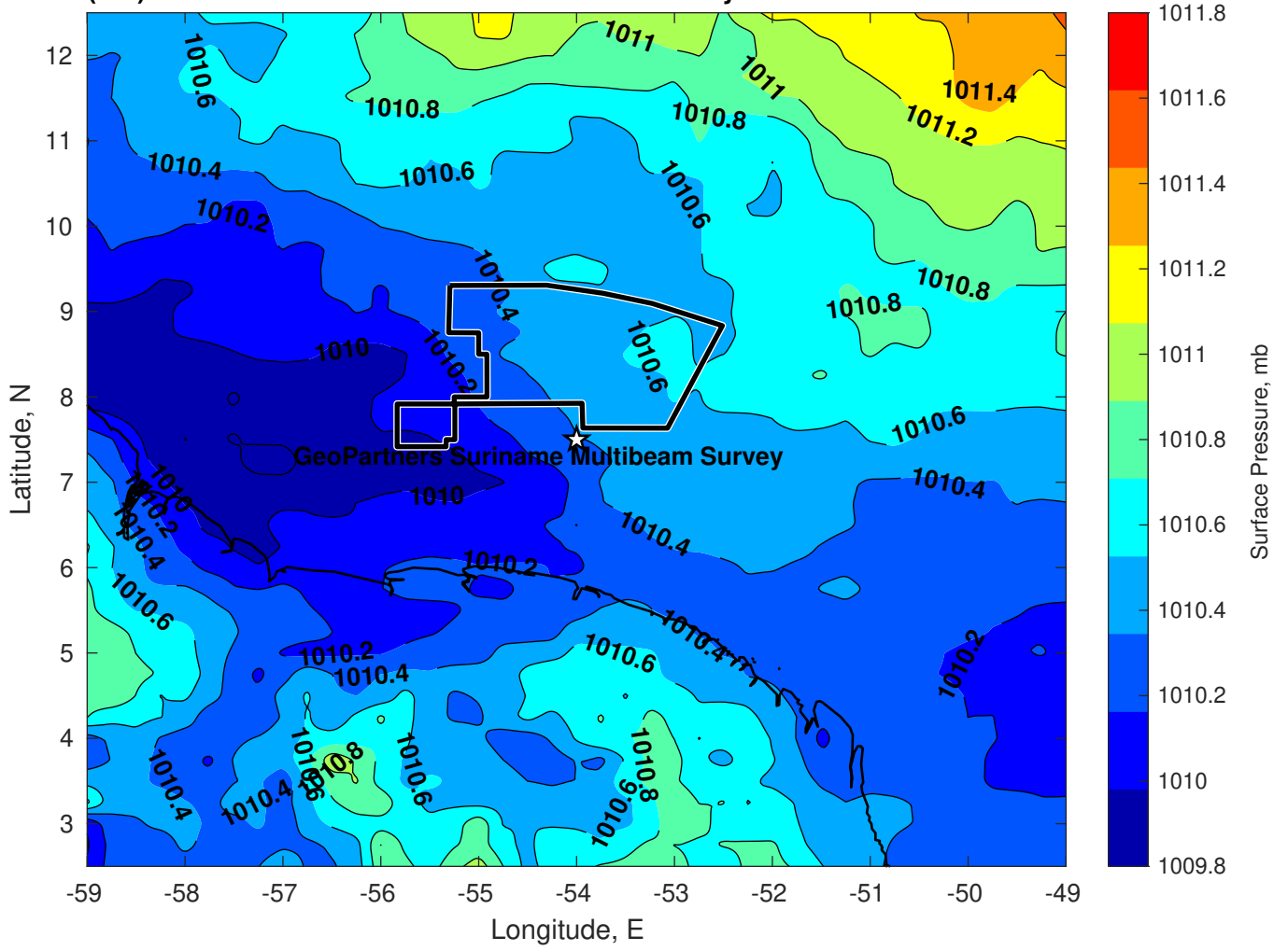
Surface Pressure (mb) for GeoPartners Suriname Multibeam Survey at 14-Nov-2024 12:00:00
