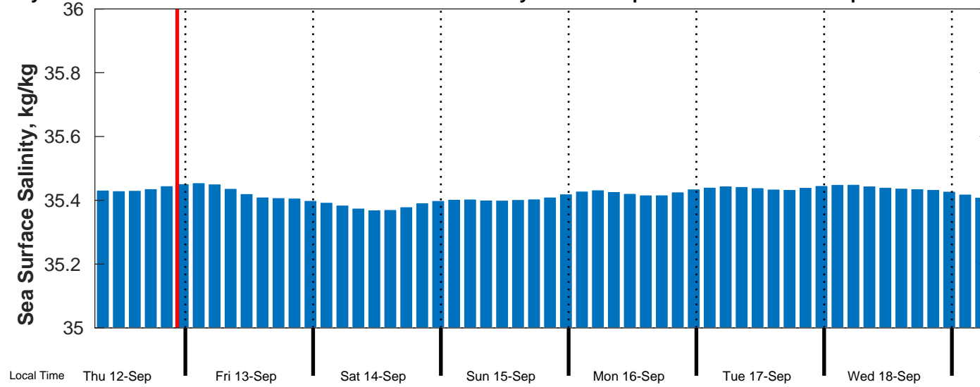
Sea Surface Salinity Forecast for GeoPartners Suriname Multibeam Survey from 13-Sep-2024 00:00:00 to 20-Sep-2024 00:00:00
