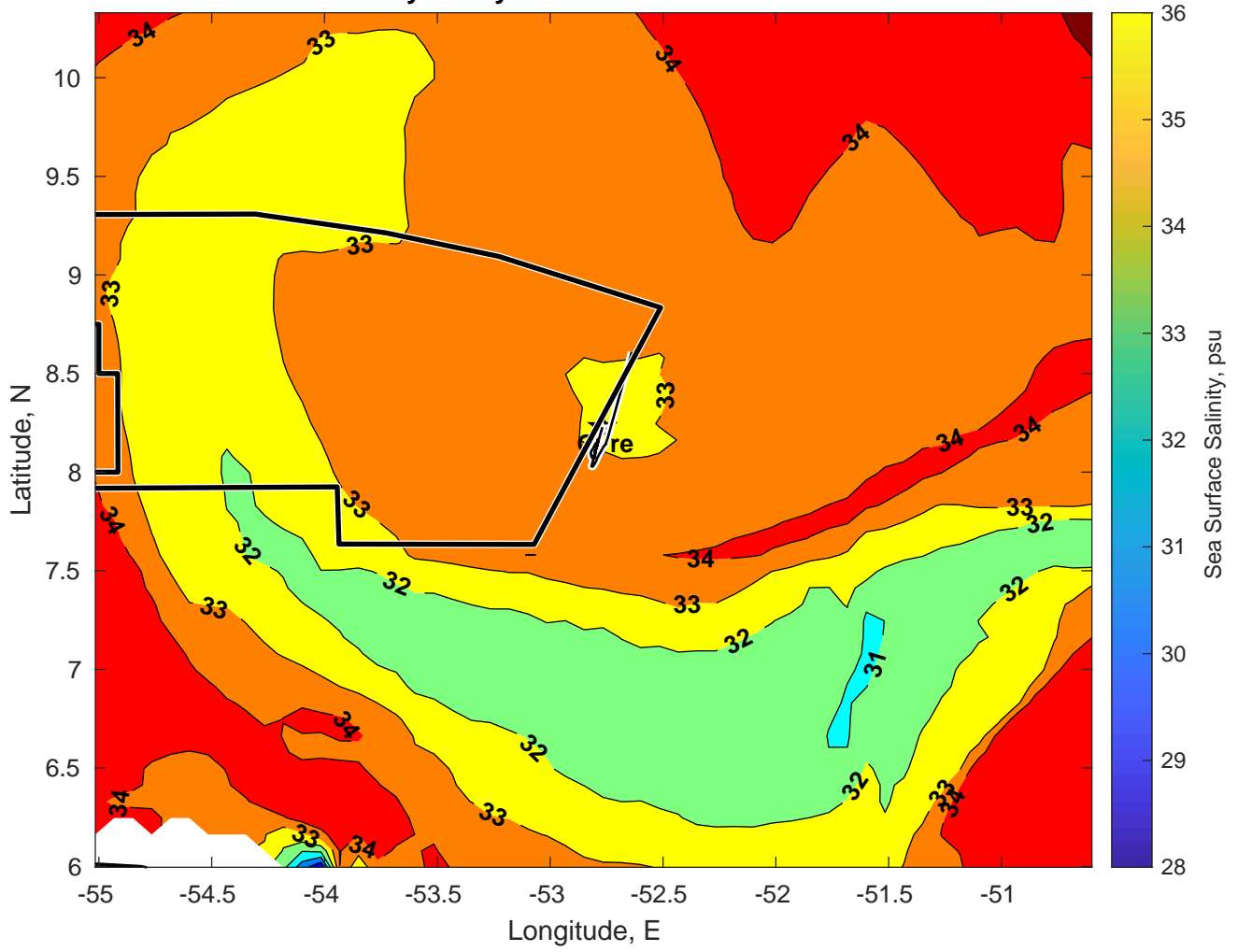
Surface Salinity for Gyre at 25-Jul-2024 00:00:00
