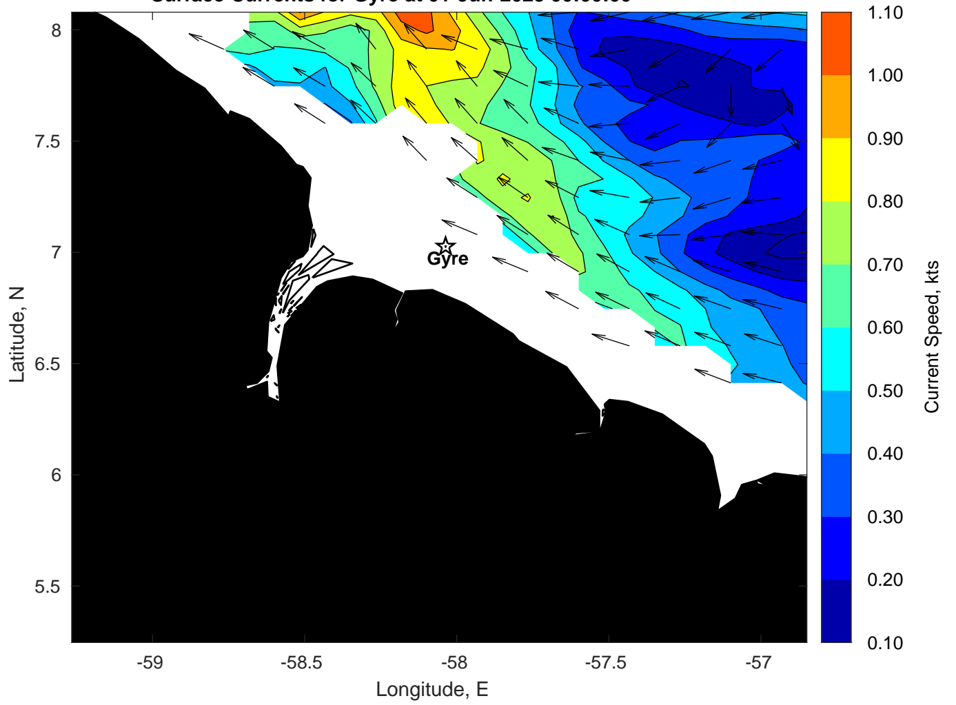
Surface Currents for Gyre at 01-Jun-2023 00:00:00
