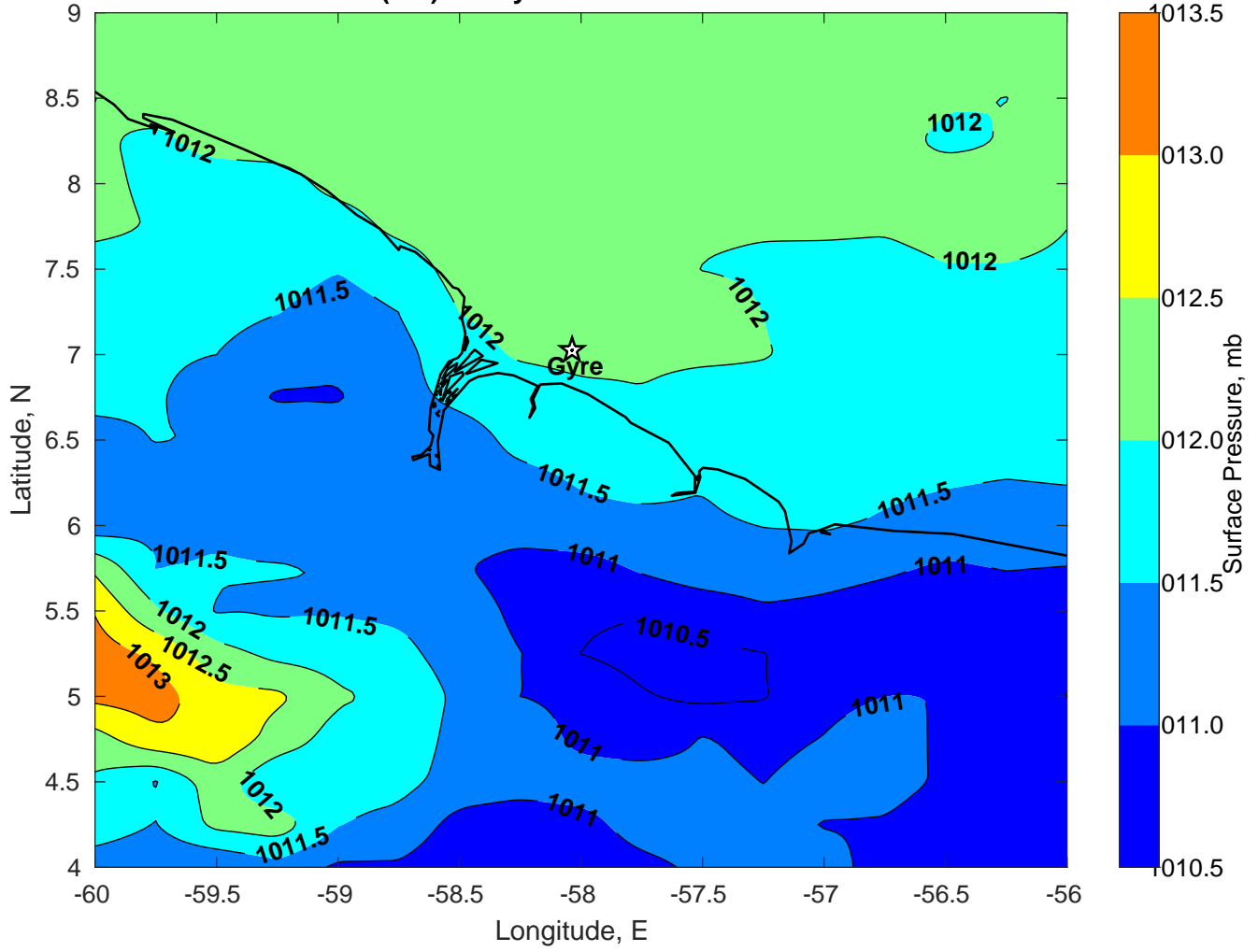
Surface Pressure (mb) for Gyre at 01-Jun-2023 18:00:00
