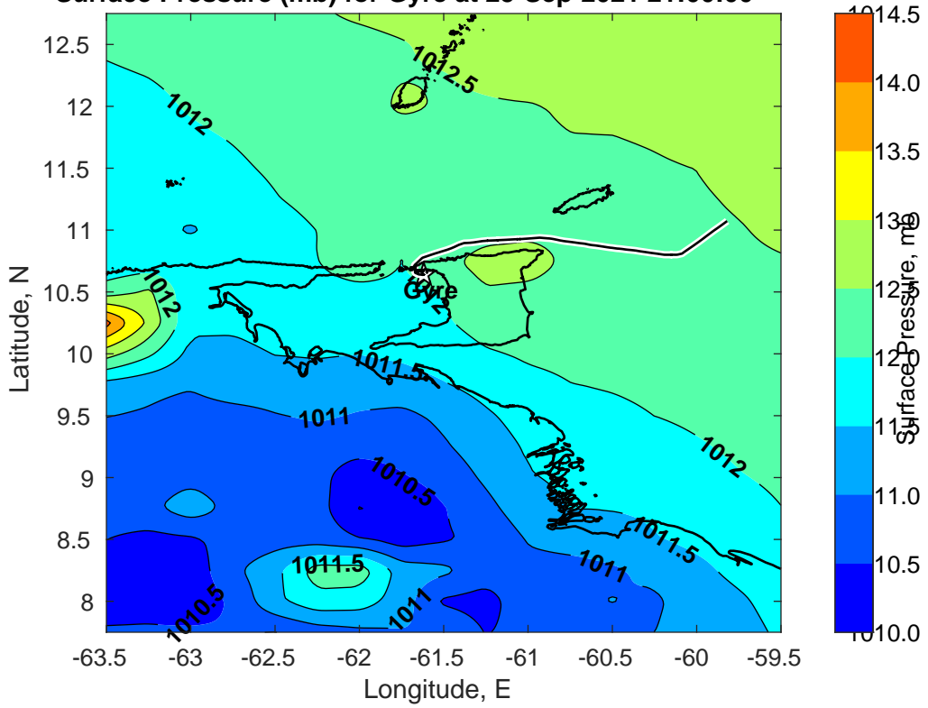
Surface Pressure (mb) for Gyre at 25-Sep-2021 21:00:00
