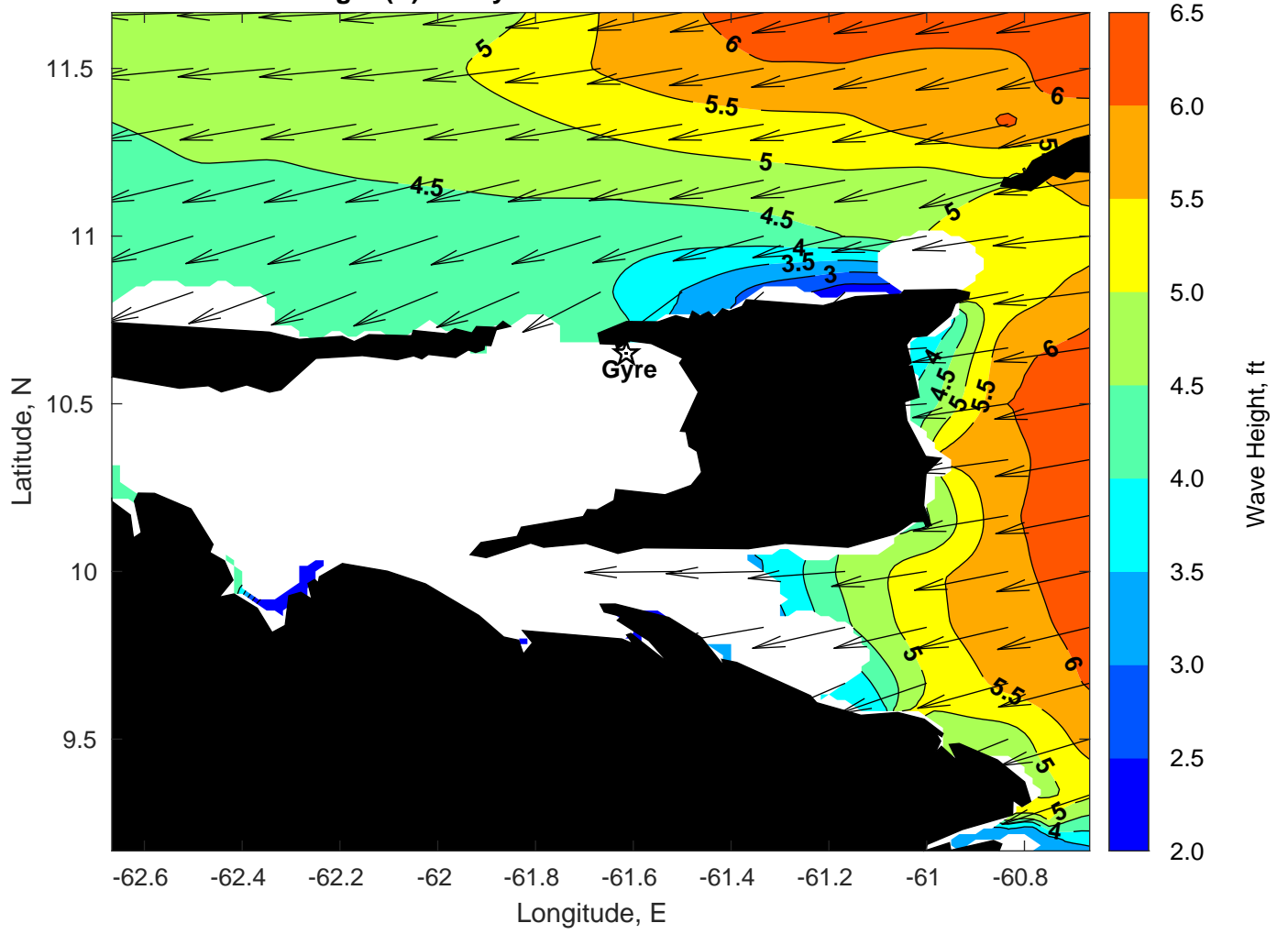
Wave Height (ft) for Gyre at 08-Feb-2023 18:00:00
