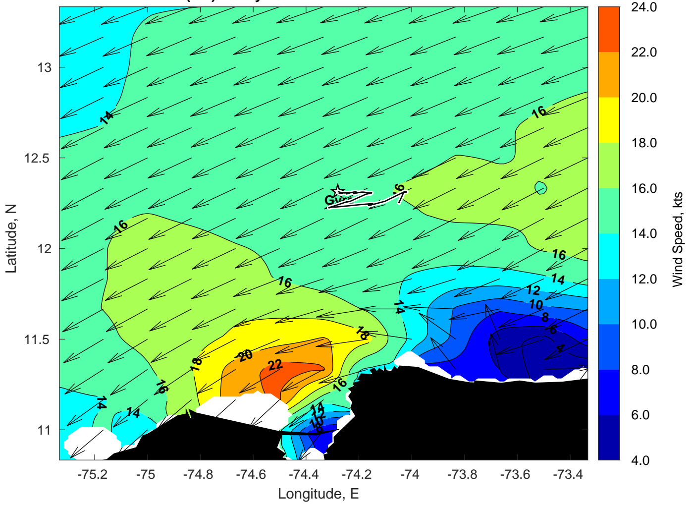
Winds (kts) for Gyre at 01-Oct-2023 00:00:00
