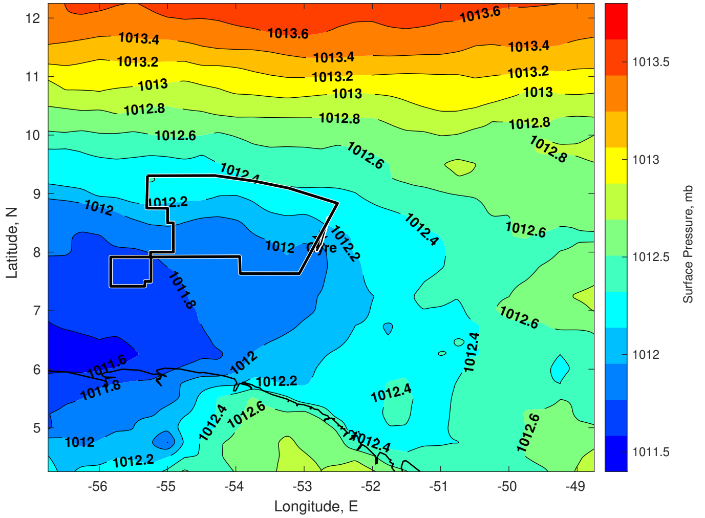
Surface Pressure (mb) for Gyre at 27-Jul-2024 06:00:00
