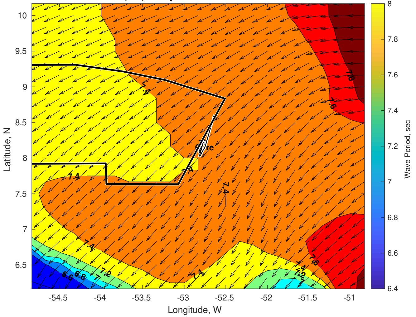
Wave Period (sec) for Gyre at 25-Jul-2024 12:00:00
