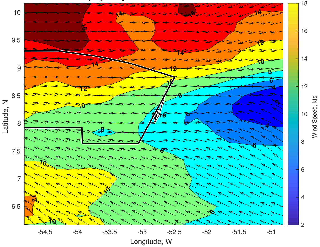
Winds (kts) for Gyre at 25-Jul-2024 12:00:00
