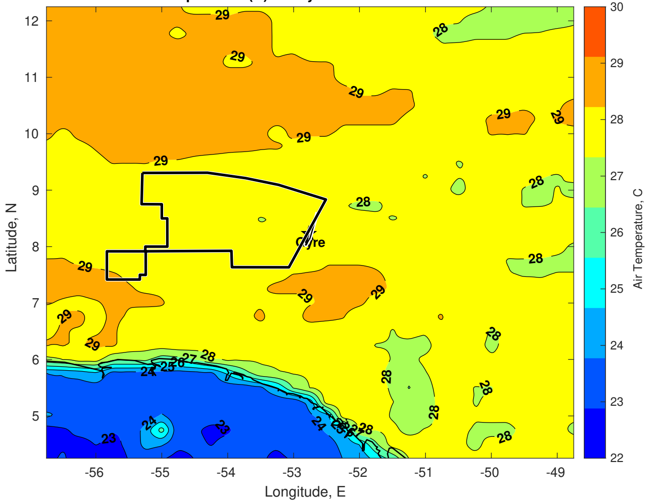
Air Temperature (C) for Gyre at 25-Jul-2024
