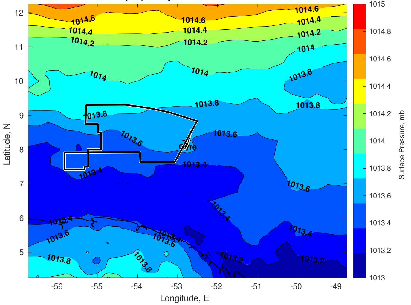
Surface Pressure (mb) for Gyre at 26-Jul-2024 06:00:00
