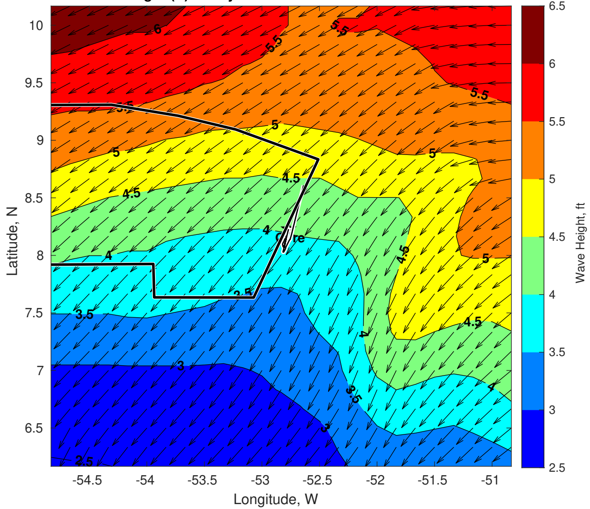
Wave Height (ft) for Gyre at 25-Jul-2024 12:00:00
