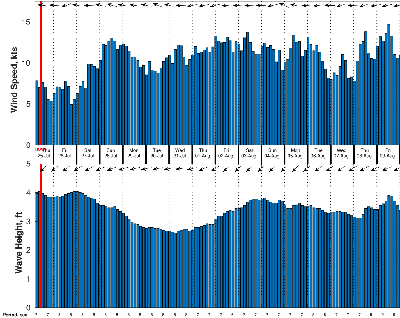
Wind & Wave Forecast for Gyre from 25-Jul-2024 05:00:00 to 10-Aug-2024 05:00:00
