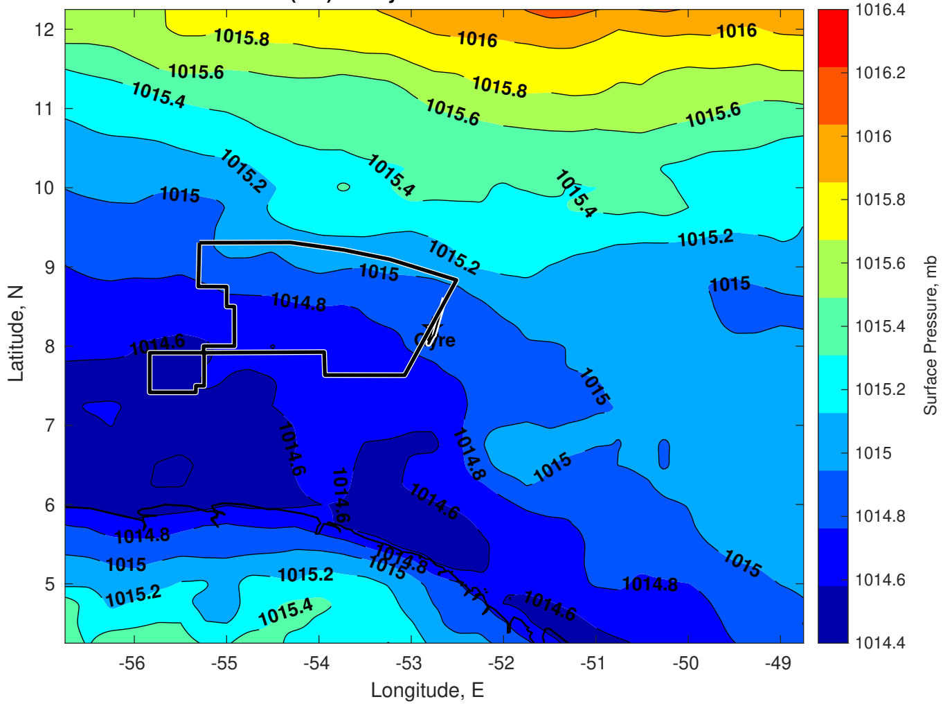
Surface Pressure (mb) for Gyre at 25-Jul-2024 06:00:00
