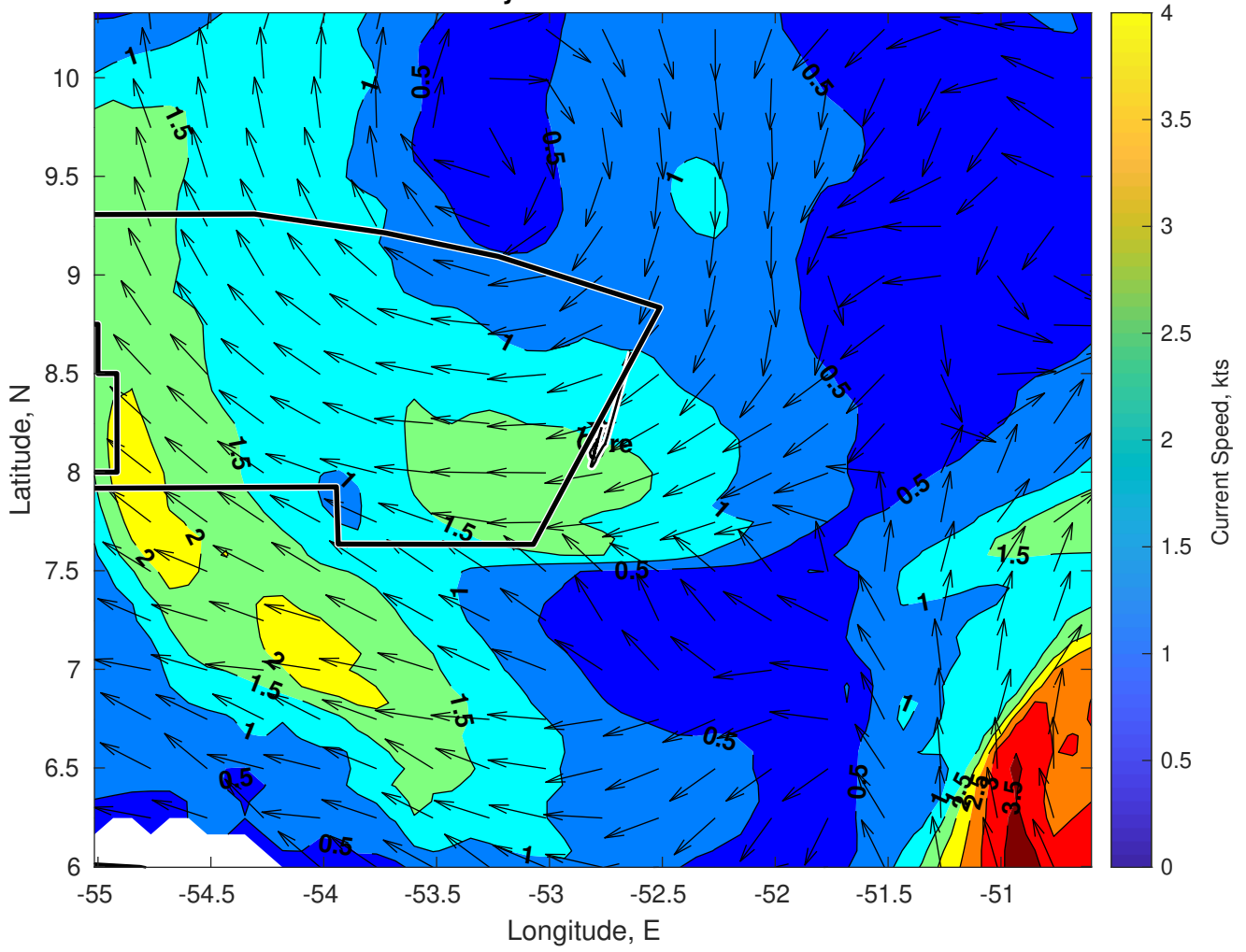
Surface Currents for Gyre at 25-Jul-2024 00:00:00
