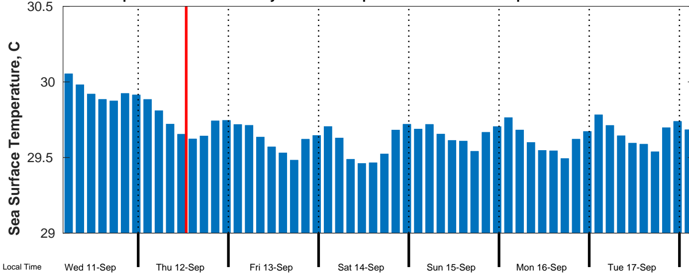
Sea Surface Temperature Forecast for Gyre from 12-Sep-2024 00:00:00 to 19-Sep-2024 00:00:00
