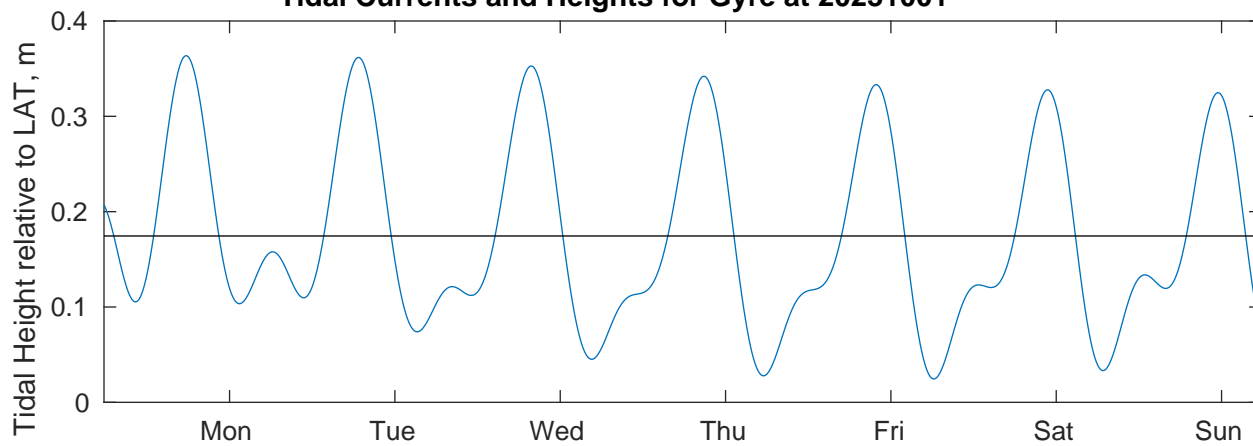
Tidal Currents and Heights for Gyre at 20231001
