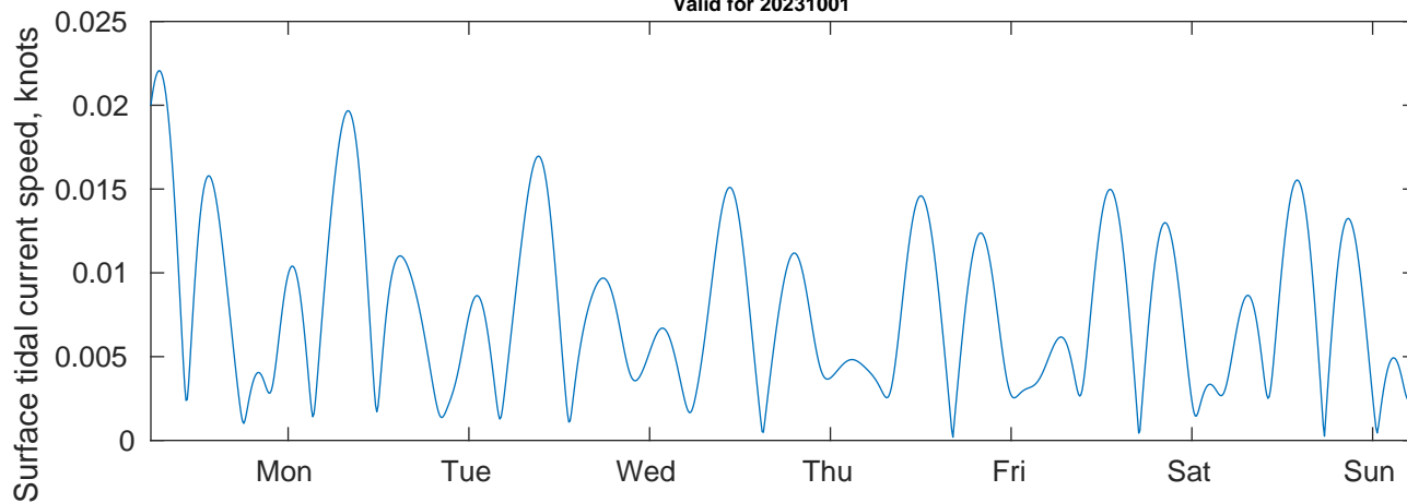
Tidal Currents and Heights for Gyre at 20231001
