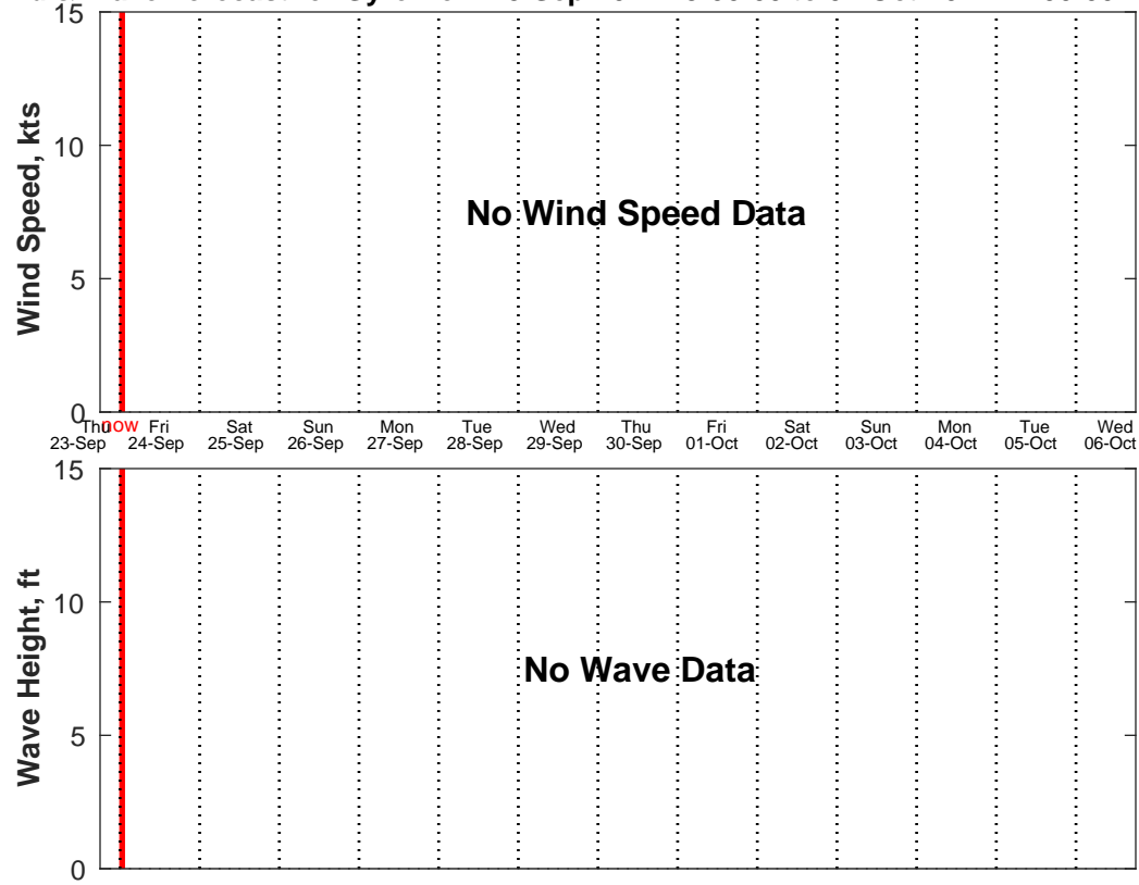
Wind & Wave Forecast for Gyre from 23-Sep-2021 18:00:00 to 07-Oct-2021 12:00:00
