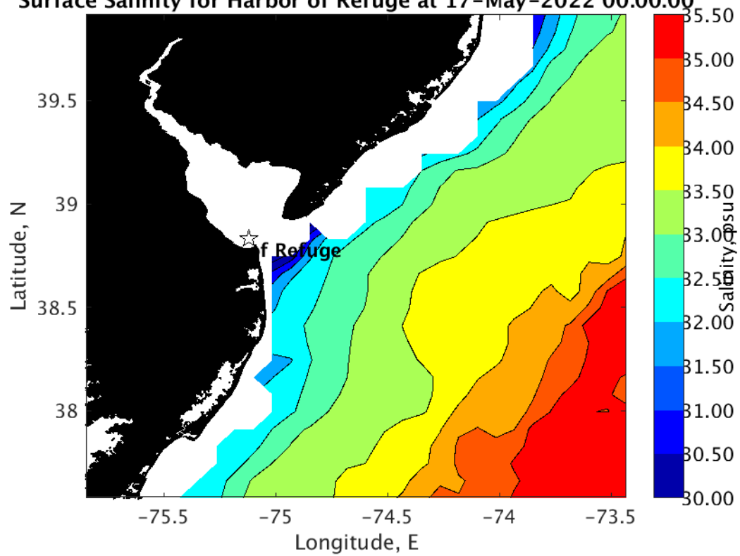
Surface Salinity for Harbor of Refuge at 17-May-2022 00:00:00
