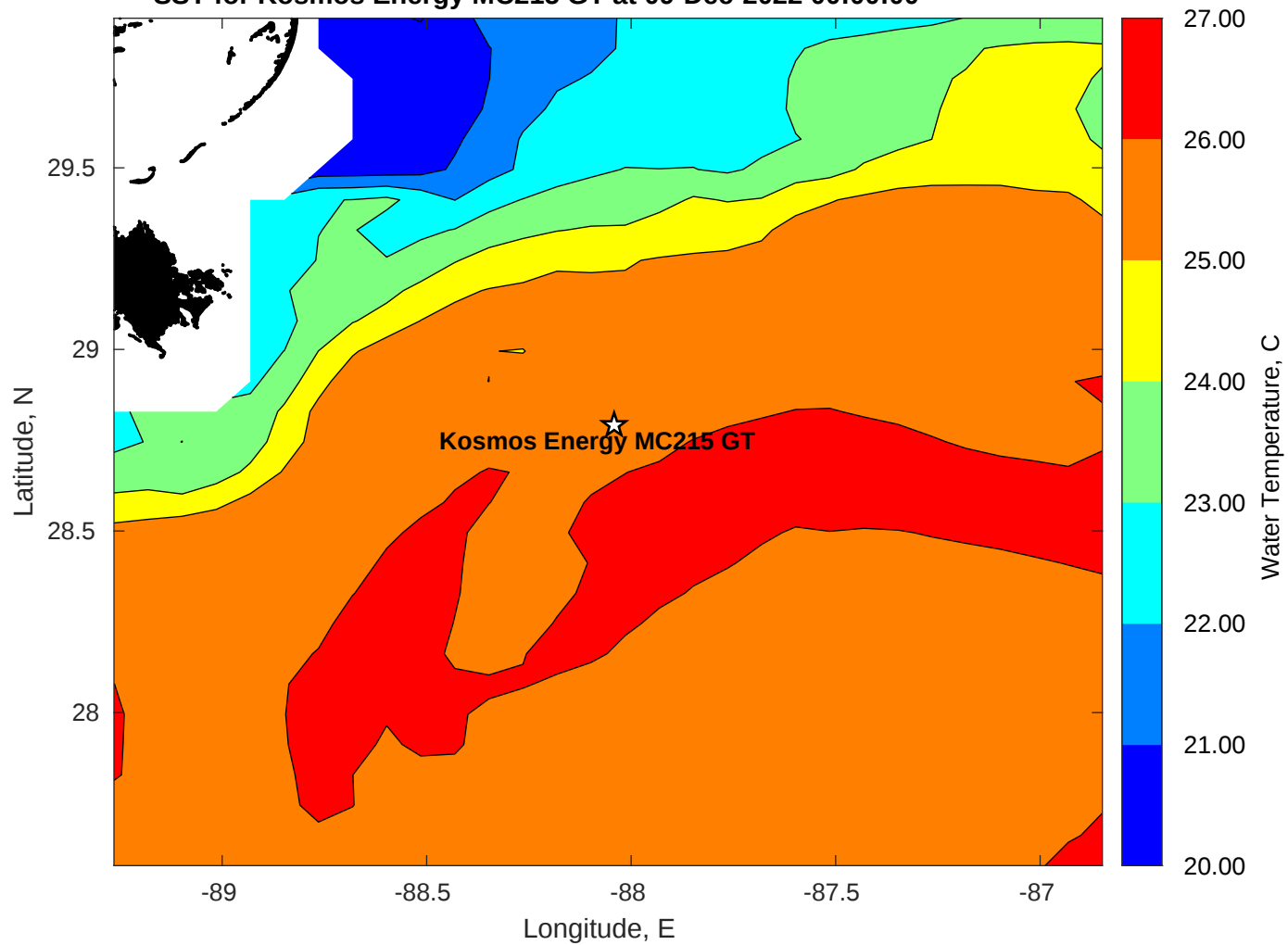
SST for Kosmos Energy MC215 GT at 09-Dec-2022 00:00:00
