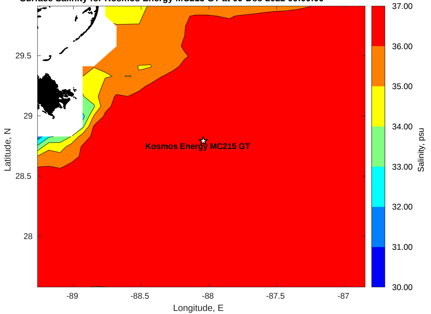
Surface Salinity for Kosmos Energy MC215 GT at 09-Dec-2022 00:00:00
