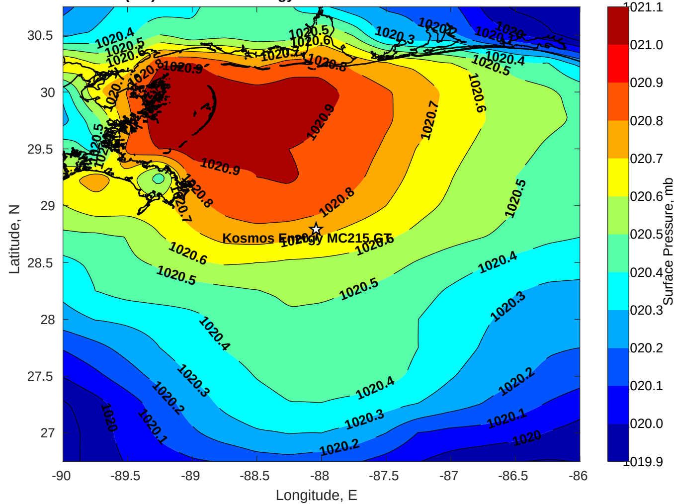
Surface Pressure (mb) for Kosmos Energy MC215 GT at 10-Dec-2022 18:00:00
