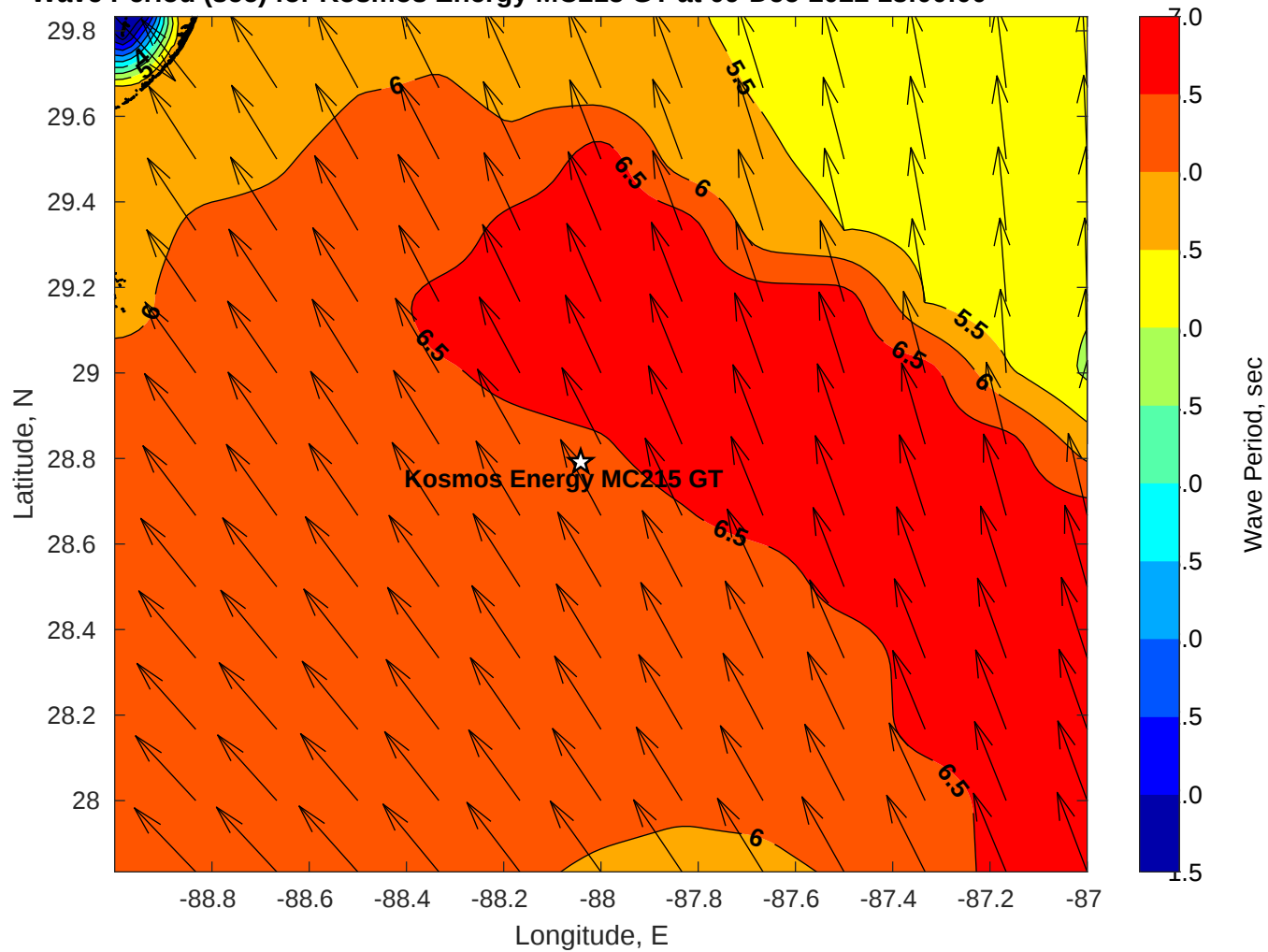
Wave Period (sec) for Kosmos Energy MC215 GT at 09-Dec-2022 18:00:00
