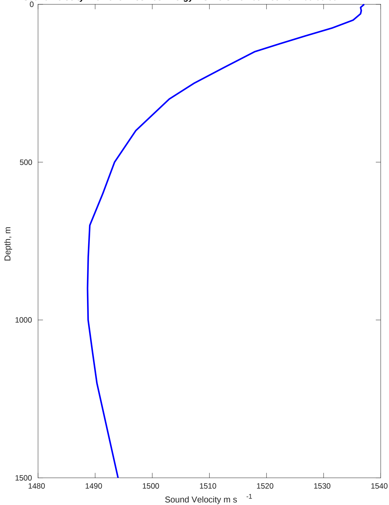
Sound Velocity Profile for Kosmos Energy MC215 GT on 09-Dec-2022 00:00:00
