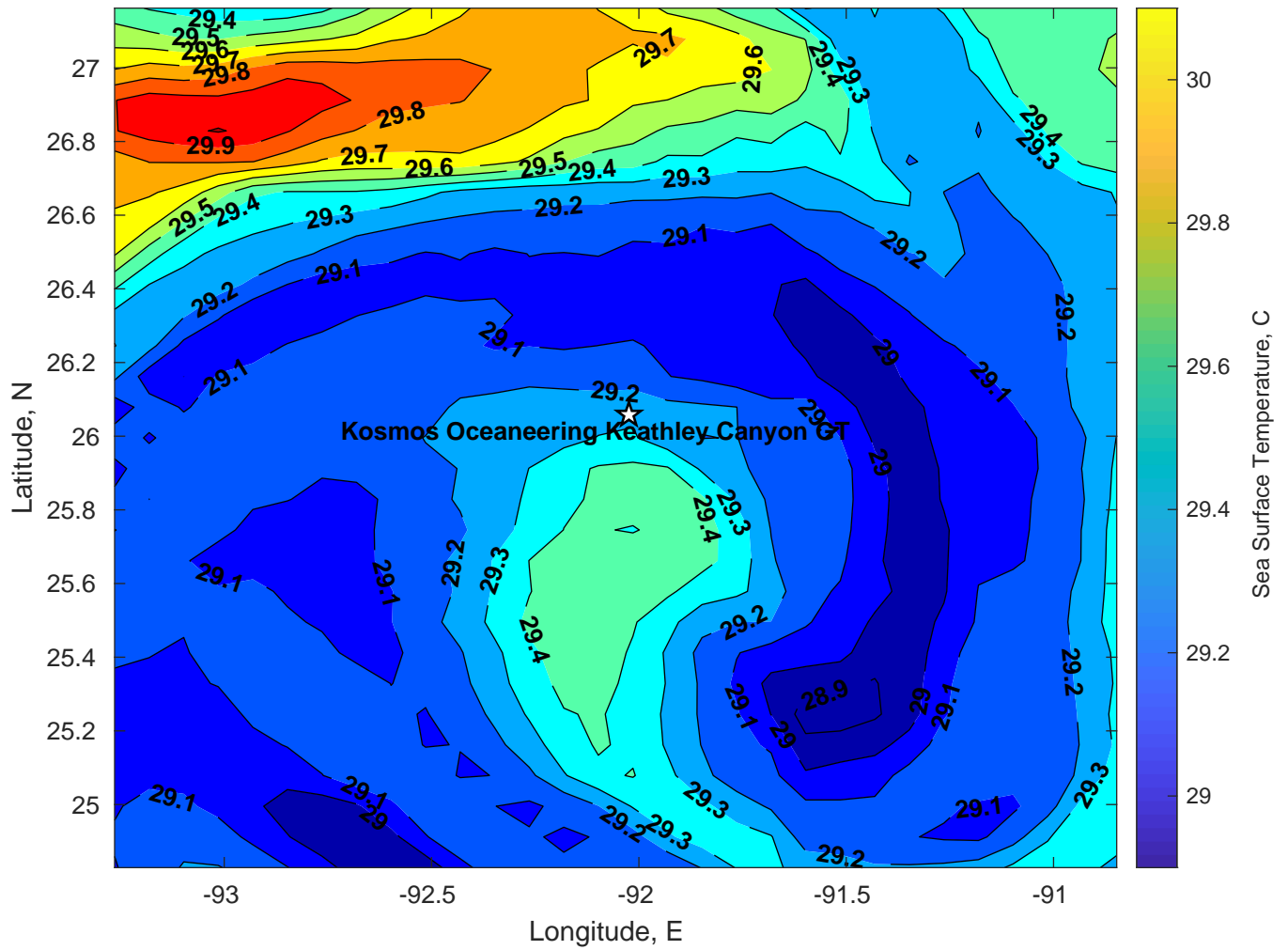
SST for Kosmos Oceaneering Keathley Canyon GT at 30-Jun-2024 00:00:00
