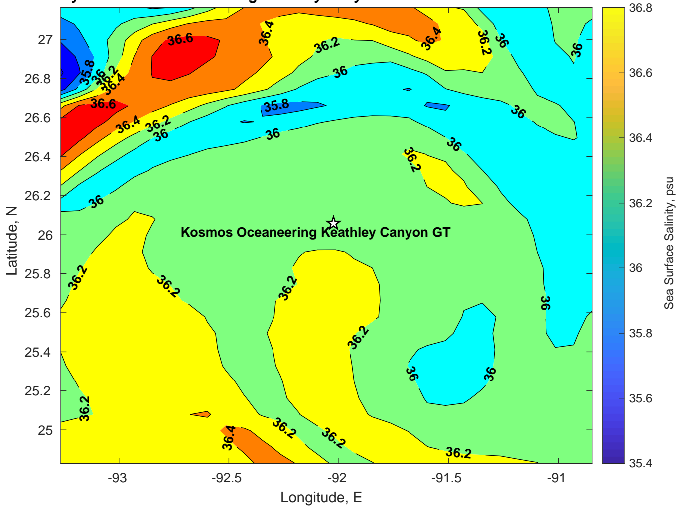
Surface Salinity for Kosmos Oceaneering Keathley Canyon GT at 30-Jun-2024 00:00:00
