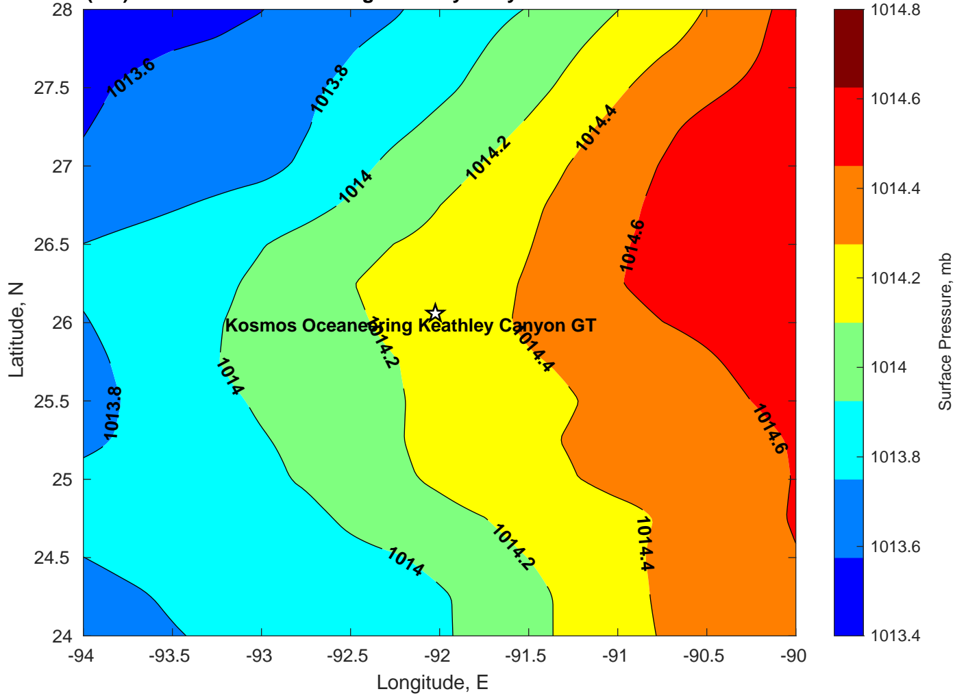
Surface Pressure (mb) for Kosmos Oceanering Keathley Canyon GT at 03-Jul-2024 06:00:00
