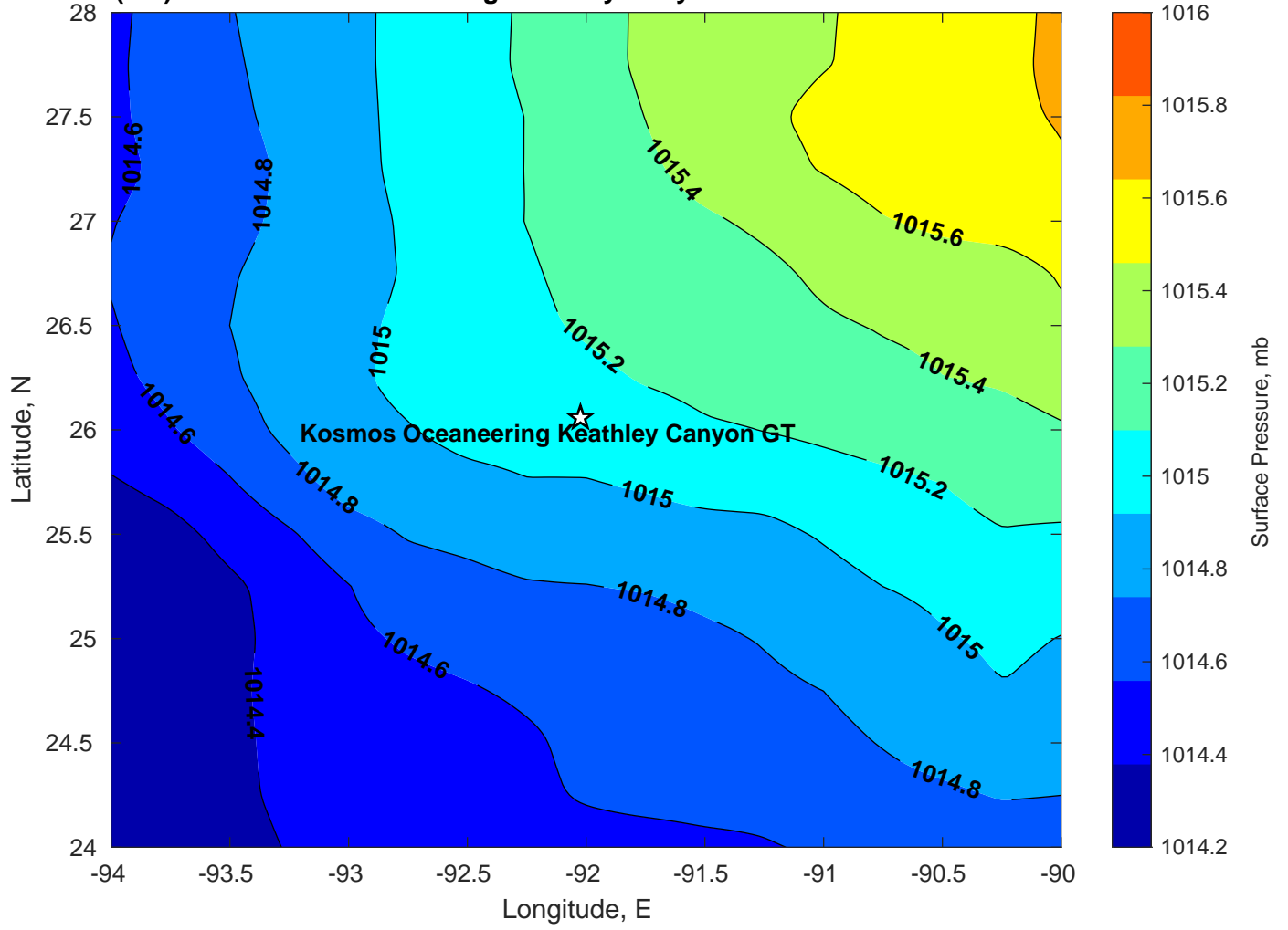
Surface Pressure (mb) for Kosmos Oceaneering Keathley Canyon GT at 04-Jul-2024 06:00:00
