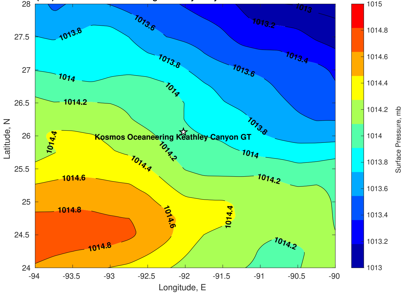
Surface Pressure (mb) for Kosmos Oceaneering Keathley Canyon GT at 02-Jul-2024 06:00:00
