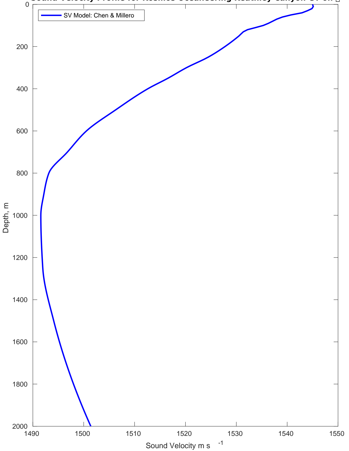
Sound Velocity Profile for Kosmos Oceaoneering Keathley Canyon GT on [ ]
