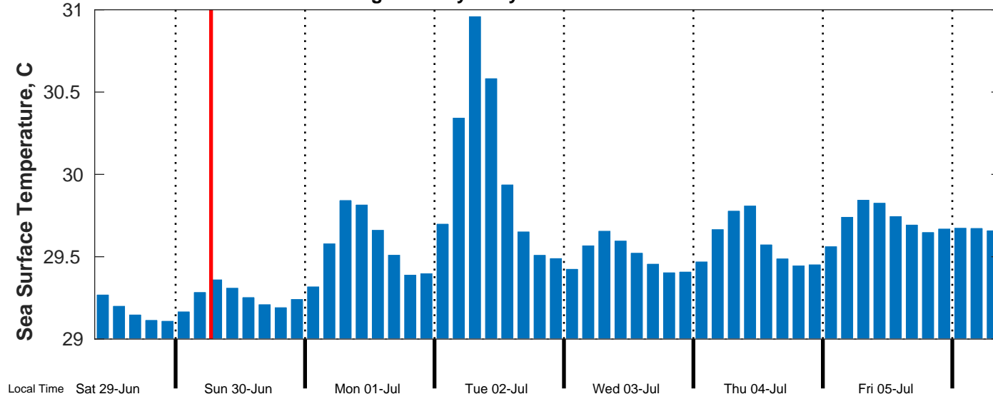
Sea Surface Temperature Forecast for Kosmos Oceaneering Keathley Canyon GT from 30-Jun-2024 00:00:00 to 07-Jul-2024 00:00:00
