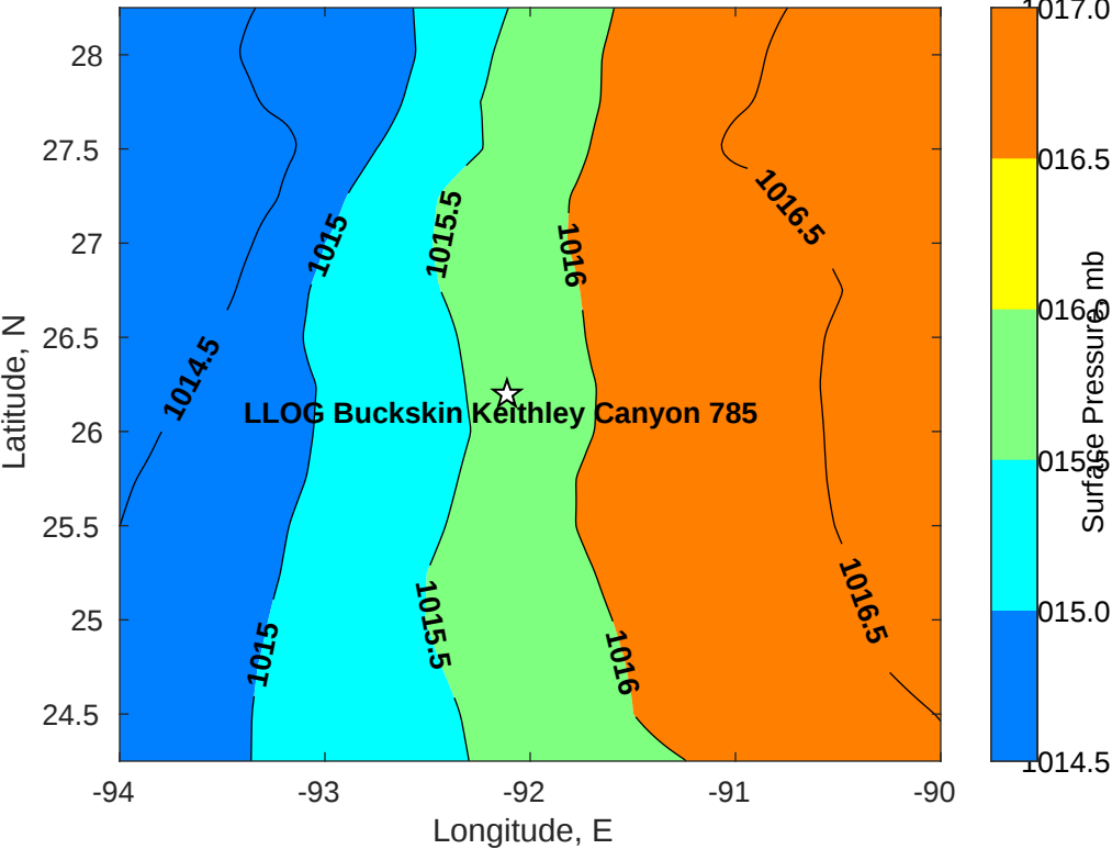
Surface Pressure (mb) for LLOG Buckskin Keithley Canyon 785 at 01-Jul-2022 00:00:00
