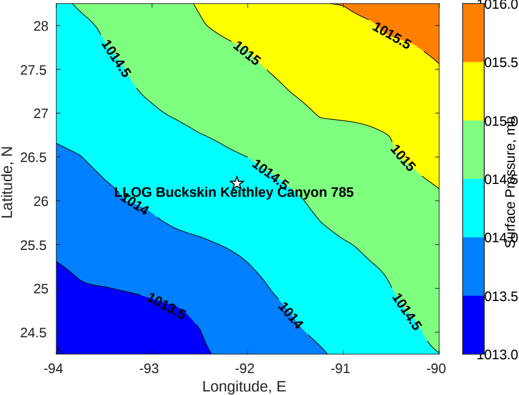
Surface Pressure (mb) for LLOG Buckskin Keithley Canyon 785 at 02-Jul-2022 21:00:00
