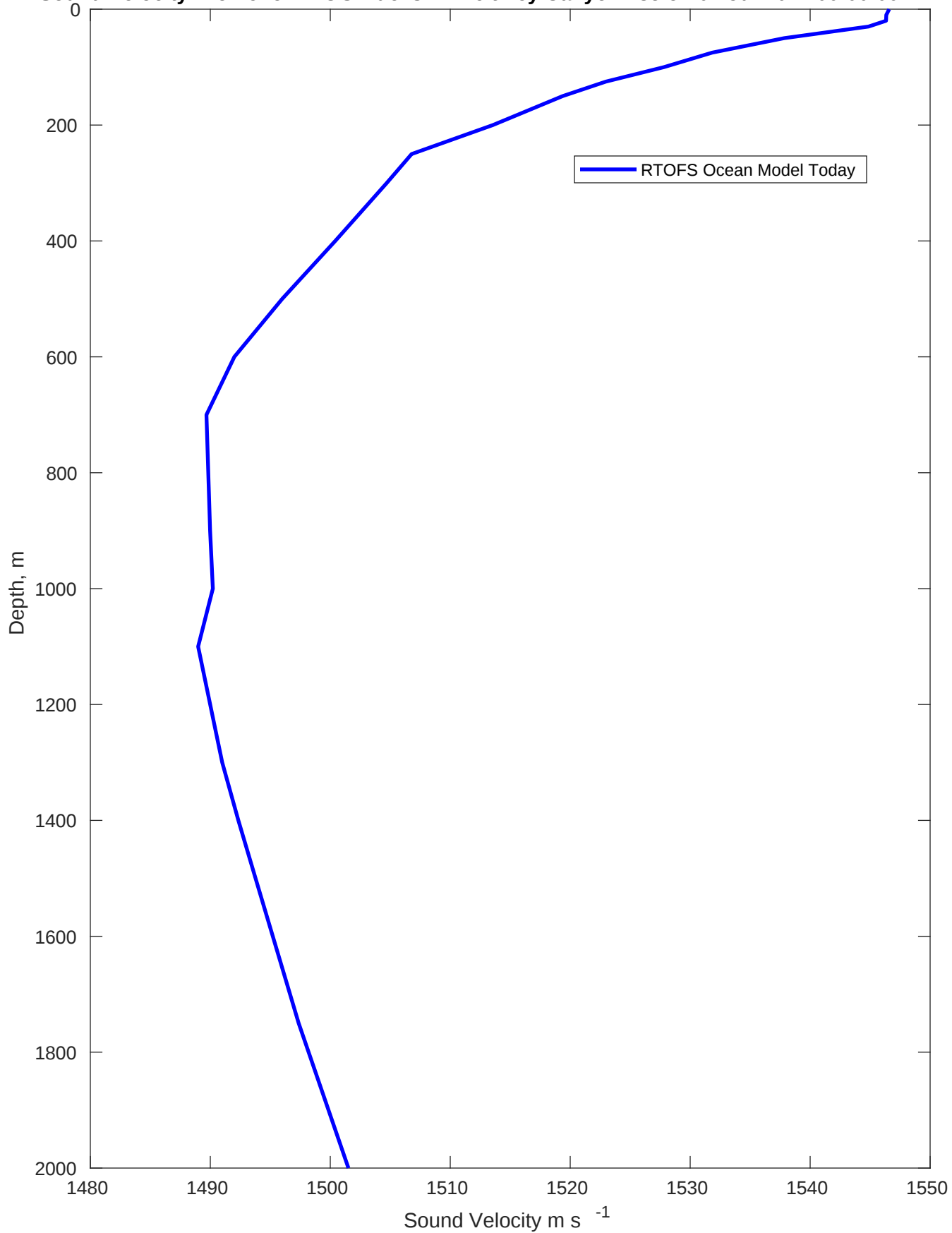
Sound Velocity Profile for LLOG Buckskin Keithley Canyon 785 on 01-Jul-2022 00:00:00
