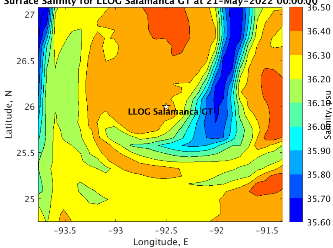
Surface Salinity for LLOG Salamanca GT at 21-May-2022 00:00:00
