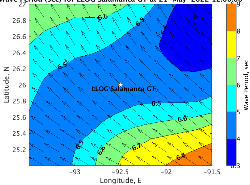
Wave Period (sec) for LLOG Salamanca GT at 21-May-2022 12:00:00
