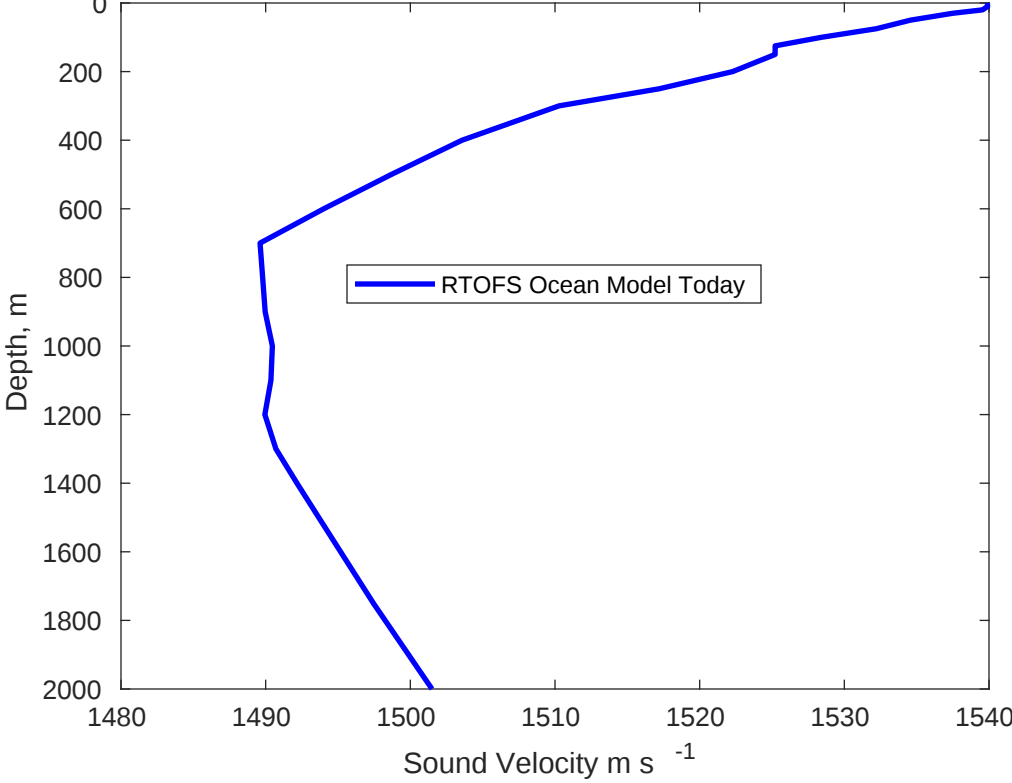
Sound Velocity Profile for LLOG Salamanca GT on 21-May-2022 00:00:00
