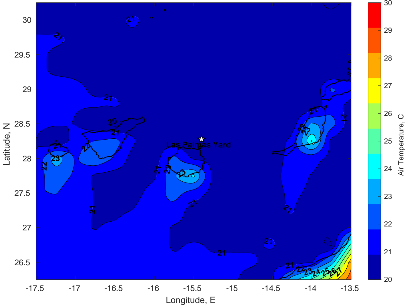
Air Temperature (C) for Las Palmas Yard at 09-May-2024
