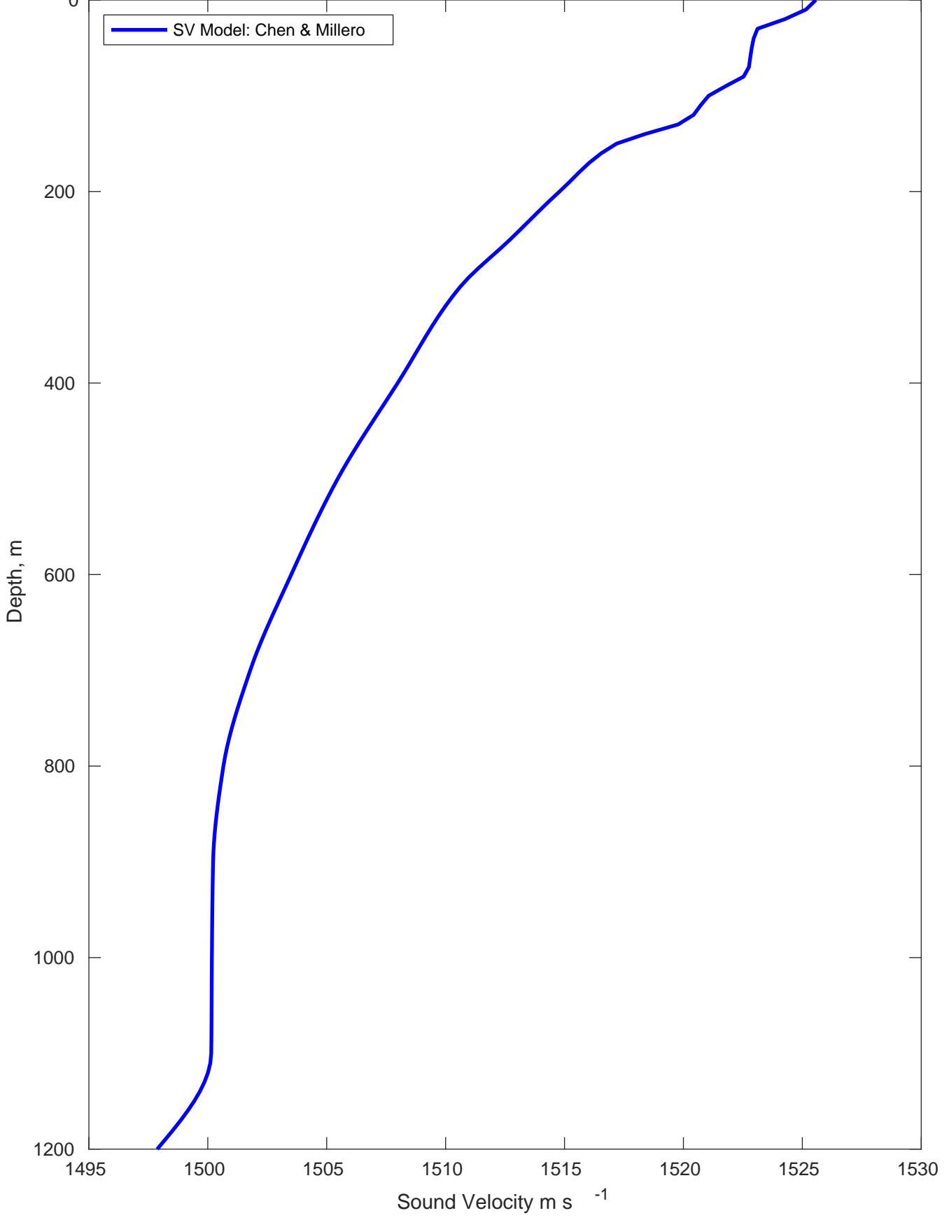
Sound Velocity Profile for Las Palmas Yard on 09-May-2024 00:00:00
