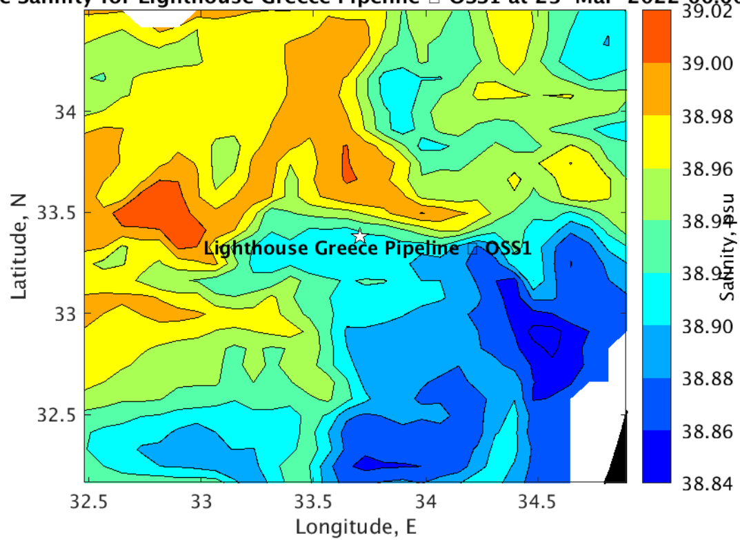
Sea Salinity for Lighthouse Greece Pipeline □ OSS1 at 23-Mar-2022 00:00:00
