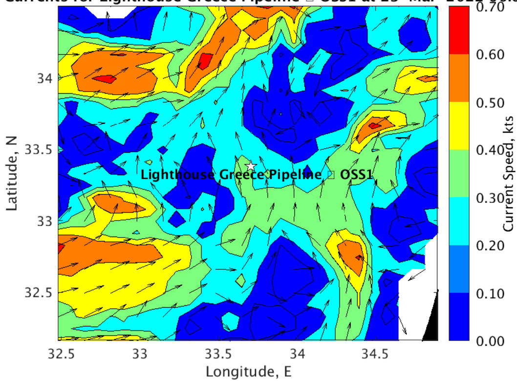
Currents for Lighthouse Greece Pipeline □ OSS1 at 23-Mar-2022 00:00:0
