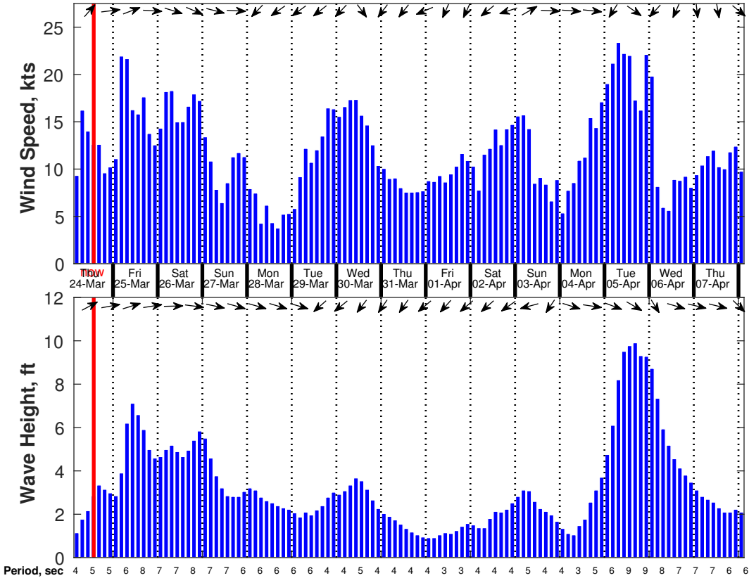
Wind & Wave Forecast for Lighthouse Greece Pipeline □ OSS1 from 23-Mar-2022 03:00:00 to 08-Apr-2022 00:00:00
